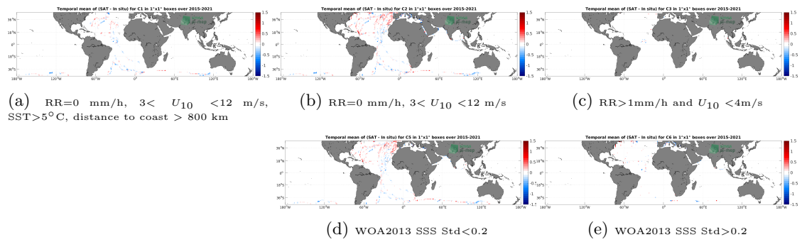
Figure 12: Temporal mean gridded over spatial boxes of size 1^\circ \times 1^\circ of \Delta SSS (SMAP SSS L3 v5 - 8-Day running (RSS) - TSG (GOSUD-Sailing-ship)) for 5 different subdatasets corresponding to: RR=0 mm/h, 3 < U_{10} < 12 m/s, SST > 5°C, distance to coast > 800 km (a), RR=0 mm/h, 3 < U_{10} < 12 m/s (b), RR > 1mm/h and U_{10} < 4 m/s (c), WOA2013 SSS Std < 0.2 (d), WOA2013 SSS Std > 0.2 (e).
