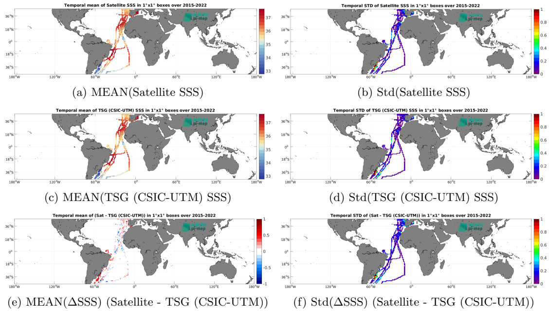
Figure 6: Temporal mean (left) and Std (right) of SSS from SMAP SSS L3 v5 - 8-Day running (RSS) (top), TSG (CSIC-UTM) (middle), and of \Delta SSS (Satellite - TSG (CSIC-UTM)). Only match-up pairs are used to generate these maps.
