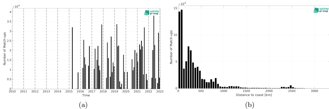
Figure 1: Number of match-ups between TSG (CSIC-UTM) and SMAP SSS L3 v5 - 8-Day running (RSS) SSS as a function of time (a) and as function of the distance to coast (b) over the Mid-Low Latitudes 45N-45S Pi-MEP region and for the full satellite product period.
