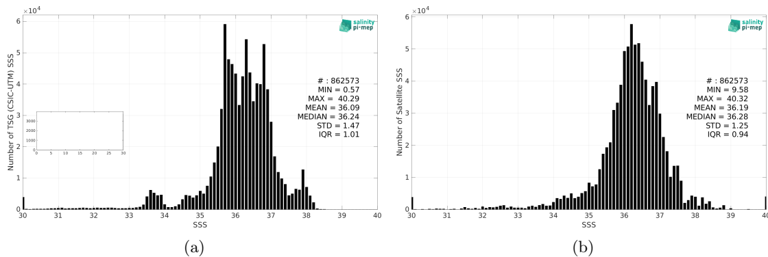
Figure 2: Histograms of SSS from TSG (CSIC-UTM) (a) and SMAP SSS L3 v5 - 8-Day running (RSS) (b) considering all match-up pairs per bins of 0.1 over the Mid-Low Latitudes 45N-45S Pi-MEP region and for the full satellite product period.
