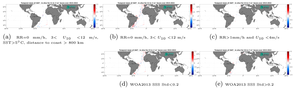
Figure 12: Temporal mean gridded over spatial boxes of size 1^\circ \times 1^\circ of \Delta SSS (SMAP SSS L3 v5 - 8-Day running (RSS) - TSG (CSIC-UTM)) for 5 different subdatasets corresponding to:RR=0 mm/h, 3 < U_{10} < 12 m/s, SST >5^\circ C, distance to coast > 800 km (a), RR=0 mm/h, 3 < U_{10} < 12 m/s (b), RR >1 mm/h and U_{10} < 4 m/s (c), WOA2013 SSS Std <0.2 (d), WOA2013 SSS Std >0.2 (e).
