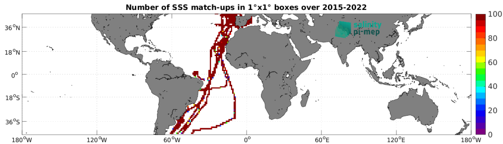
Figure 4: Number of SSS match-ups between TSG (CSIC-UTM) SSS and the SMAP SSS L3 v5 - 8-Day running (RSS) SSS product for the Mid-Low Latitudes 45N-45S Pi-MEP region over 1^\circ \times 1^\circ boxes and for the full satellite product period.
