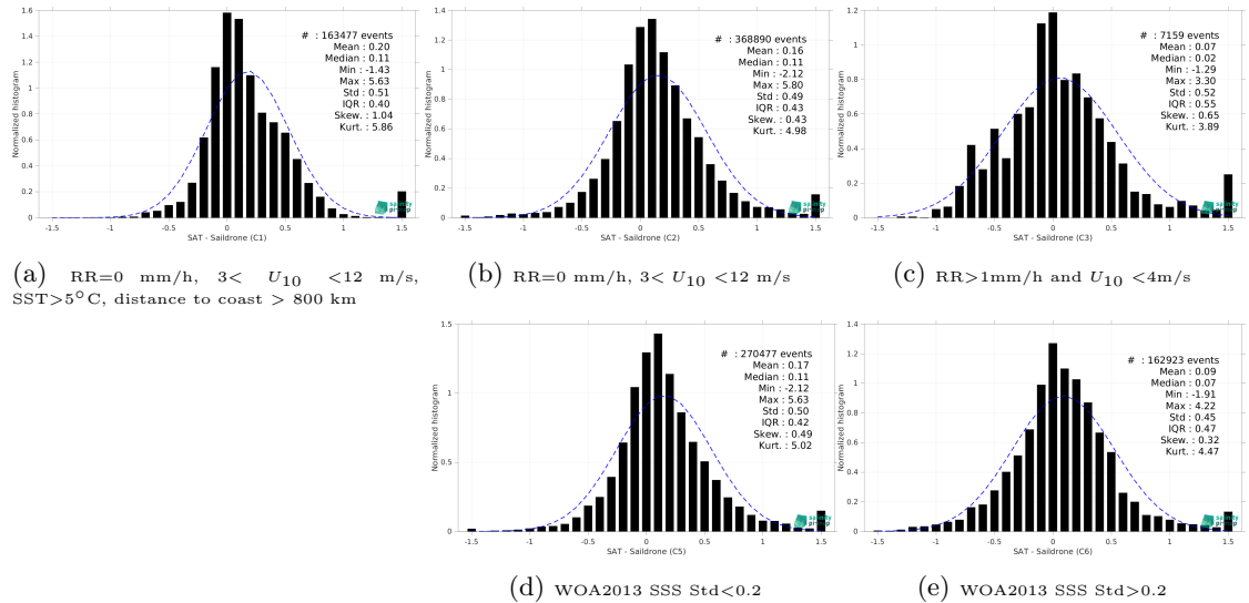
Figure 13: Normalized histogram of \Delta SSS (SMAP SSS L3 v5 - 8-Day running (RSS) - Saildrone) for 5 different subdatasets corresponding to: RR=0 mm/h, 3 < U_{10} < 12 m/s, SST >5^\circ\text{C} , distance to coast > 800 km (a), RR=0 mm/h, 3 < U_{10} < 12 m/s (b), RR >1 mm/h and U_{10} < 4 m/s (c), WOA2013 SSS Std <0.2 (d), WOA2013 SSS Std >0.2 (e).
