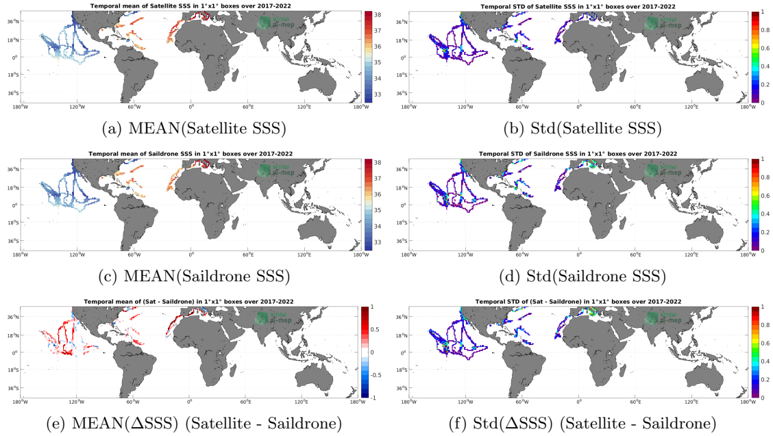
Figure 6: Temporal mean (left) and Std (right) of SSS from SMAP SSS L3 v5 - 8-Day running (RSS) (top), Saildrone (middle), and of \Delta SSS (Satellite - Saildrone). Only match-up pairs are used to generate these maps.
