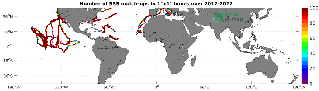
Figure 4: Number of SSS match-ups between Saildrone SSS and the SMAP SSS L3 v5 - 8-Day running (RSS) SSS product for the Mid-Low Latitudes 45N-45S Pi-MEP region over 1^\circ \times 1^\circ boxes and for the full satellite product period.
