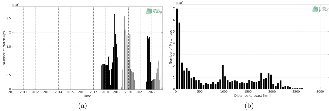
Figure 1: Number of match-ups between Saildrone and SMAP SSS L3 v5 - 8-Day running (RSS) SSS as a function of time (a) and as function of the distance to coast (b) over the Mid-Low Latitudes 45N-45S Pi-MEP region and for the full satellite product period.
