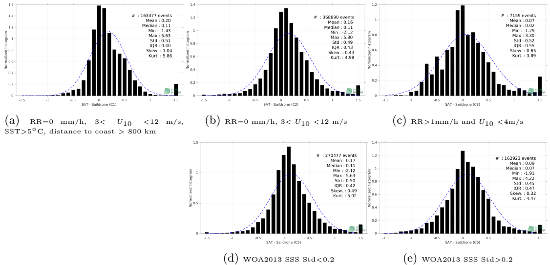
Figure 13: Normalized histogram of \Delta SSS (SMAP SSS L3 v5 - 8-Day running (RSS) - Saildrone) for 5 different subdatasets corresponding to: RR=0 mm/h, 3 < U_{10} < 12 m/s, SST>5°C, distance to coast > 800 km (a), RR=0 mm/h, 3 < U_{10} < 12 m/s (b), RR>1mm/h and U_{10} < 4 m/s (c), WOA2013 SSS Std<0.2 (d), WOA2013 SSS Std>0.2 (e).
