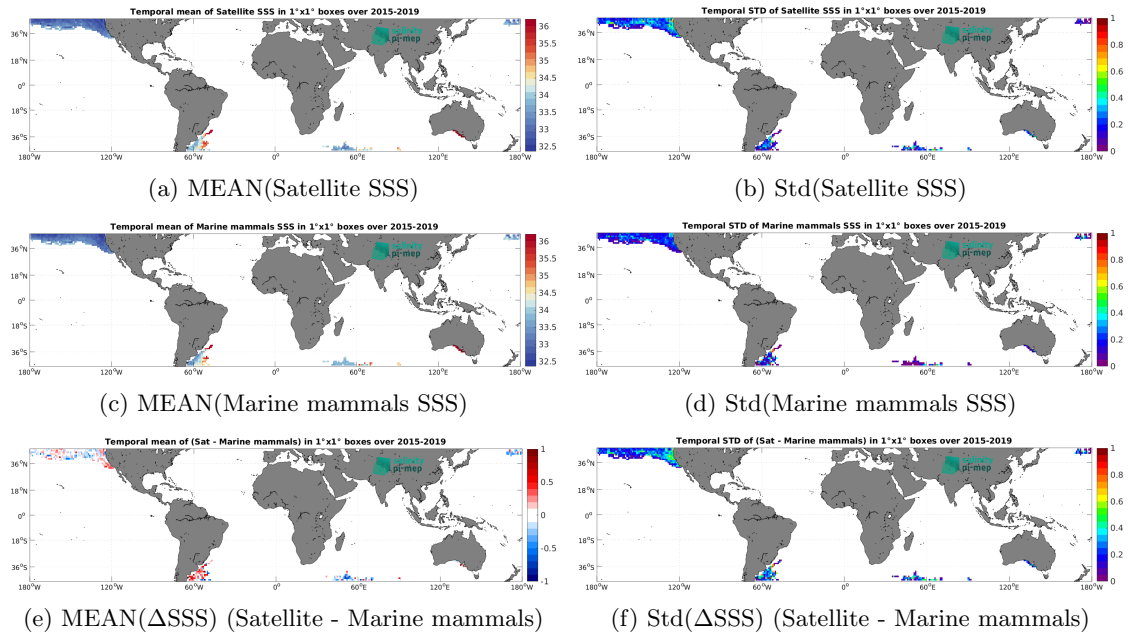
Figure 6: Temporal mean (left) and Std (right) of SSS from SMAP SSS L3 v5 - 8-Day running (RSS) (top), Marine mammals (middle), and of \Delta SSS (Satellite - Marine mammals). Only match-up pairs are used to generate these maps.
