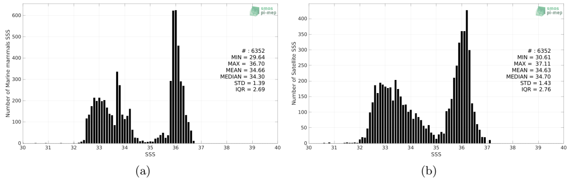
Figure 2: Histograms of SSS from Marine mammals (a) and SMAP SSS L3 v5 - 8-Day running (RSS) (b) considering all match-up pairs per bins of 0.1 over the Mid-Low Latitudes 45N-45S Pi-MEP region and for the full satellite product period.
