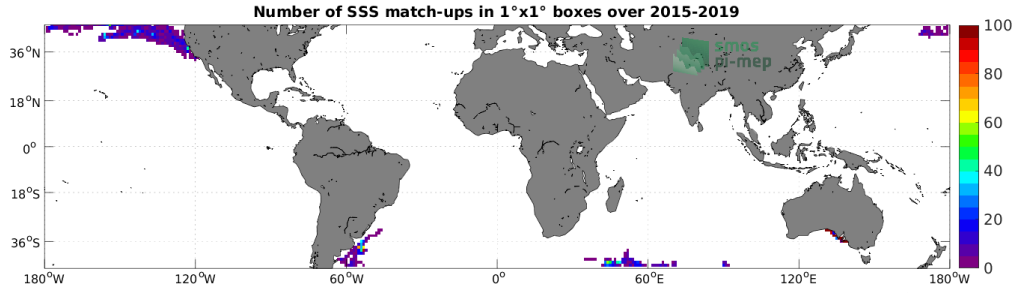
Figure 4: Number of SSS match-ups between Marine mammals SSS and the SMAP SSS L3 v5 - 8-Day running (RSS) SSS product for the Mid-Low Latitudes 45N-45S Pi-MEP region over 1^\circ \times 1^\circ boxes and for the full satellite product period.
