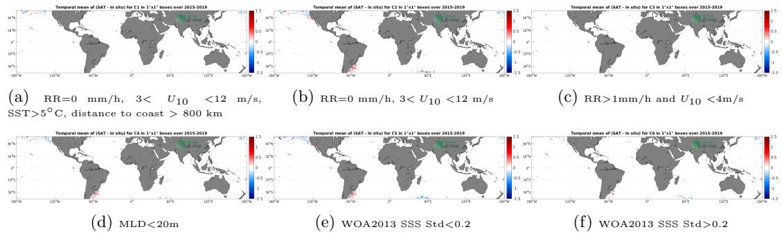
Figure 12: Temporal mean gridded over spatial boxes of size 1^\circ \times 1^\circ of \Delta SSS (SMAP SSS L3 v5 - 8-Day running (RSS) - Marine mammals) for 6 different subdatasets corresponding to:RR=0 mm/h, 3 < U_{10} < 12 m/s, SST >5^\circ\text{C} , distance to coast > 800 km (a), RR=0 mm/h, 3 < U_{10} < 12 m/s (b), RR >1 mm/h and U_{10} < 4 m/s (c),MLD <20 m (d),WOA2013 SSS Std <0.2 (e),WOA2013 SSS Std >0.2 (f).
