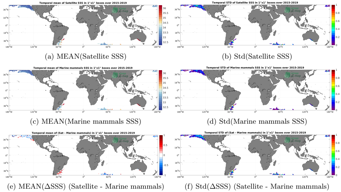
Figure 6: Temporal mean (left) and Std (right) of SSS from SMAP SSS L3 v5 - 8-Day running (RSS) (top), Marine mammals (middle), and of \Delta SSS (Satellite - Marine mammals). Only match-up pairs are used to generate these maps.
