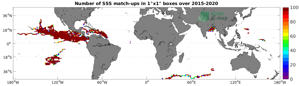
Figure 3: Number of SSS match-ups between Surface drifters SSS and the SMAP SSS L3 v5 - 8-Day running (RSS) SSS product for the Mid-Low Latitudes 45N-45S Pi-MEP region over 1^\circ \times 1^\circ boxes and for the full satellite product period.
