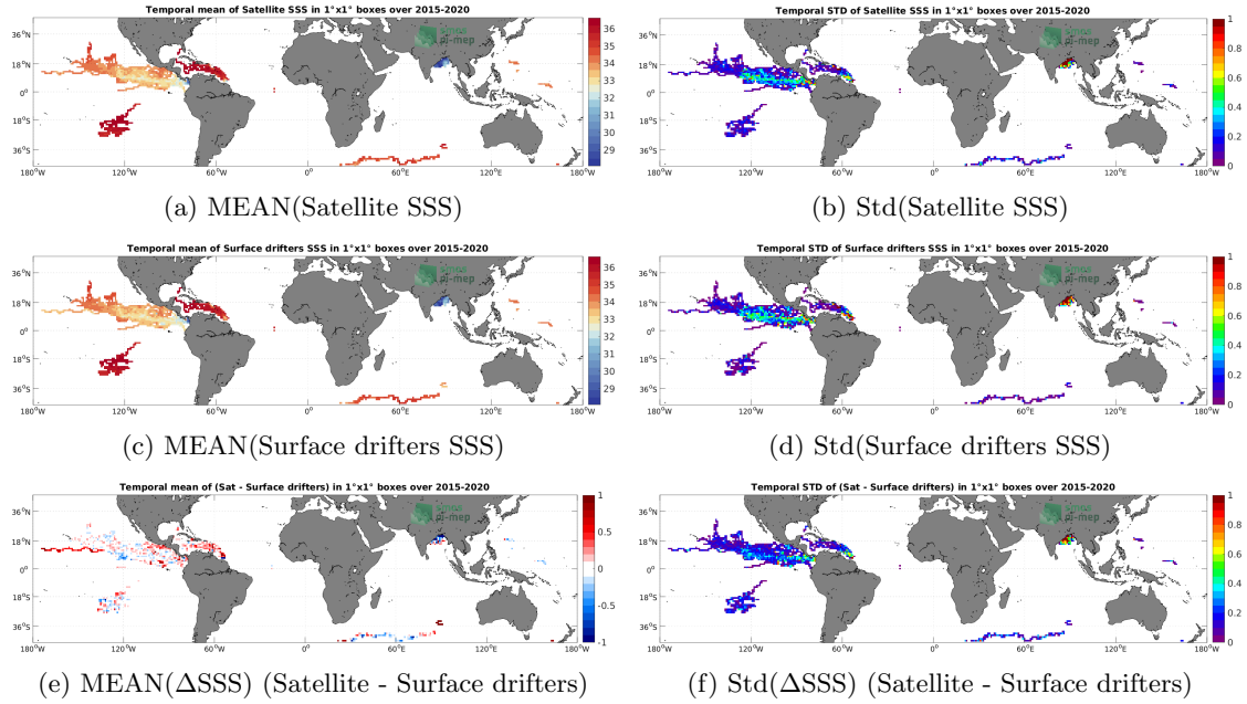
Figure 5: Temporal mean (left) and Std (right) of SSS from SMAP SSS L3 v5 - 8-Day running (RSS) (top), Surface drifters (middle), and of \Delta SSS (Satellite - Surface drifters). Only match-up pairs are used to generate these maps.
