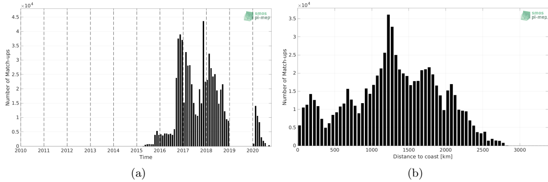
Figure 1: Number of match-ups between Surface drifters and SMAP SSS L3 v5 - 8-Day running (RSS) SSS as a function of time (a) and as function of the distance to coast (b) over the Mid-Low Latitudes 45N-45S Pi-MEP region and for the full satellite product period.
