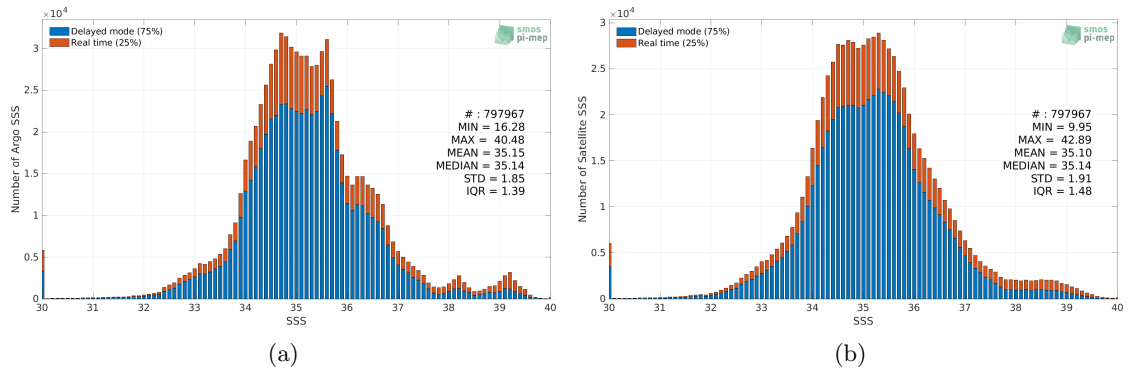
Figure 2: Histograms of SSS from Argo (a) and SMAP SSS L3 v5 - 8-Day running (RSS) (b) considering all match-up pairs per bins of 0.1 over the Mid-Low Latitudes 45N-45S Pi-MEP region and for the full satellite product period.
