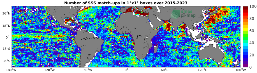
Figure 4: Number of SSS match-ups between Argo SSS and the SMAP SSS L3 v5 - 8-Day running (RSS) SSS product for the Mid-Low Latitudes 45N-45S Pi-MEP region over 1^\circ \times 1^\circ boxes and for the full satellite product period.
