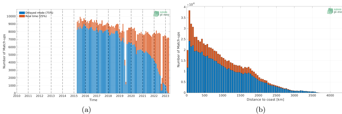
Figure 1: Number of match-ups between Argo and SMAP SSS L3 v5 - 8-Day running (RSS) SSS as a function of time (a) and as function of the distance to coast (b) over the Mid-Low Latitudes 45N-45S Pi-MEP region and for the full satellite product period.
