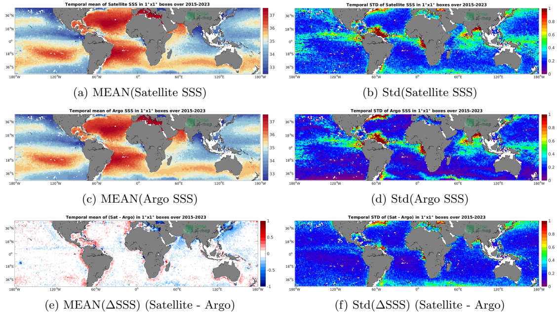
Figure 6: Temporal mean (left) and Std (right) of SSS from SMAP SSS L3 v5 - 8-Day running (RSS) (top), Argo (middle), and of \Delta SSS (Satellite - Argo). Only match-up pairs are used to generate these maps.
