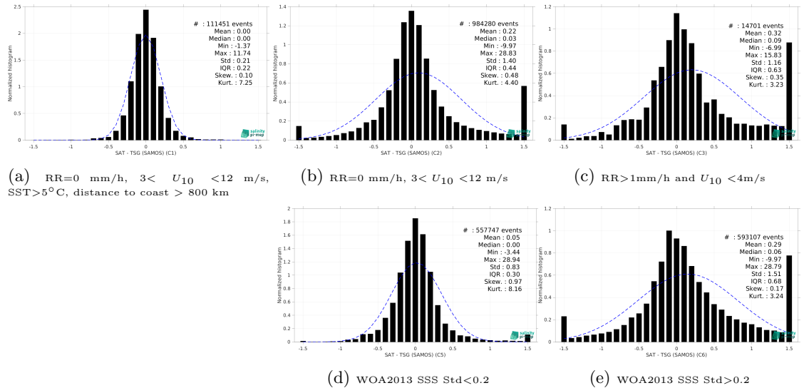
Figure 13: Normalized histogram of \Delta SSS (SMAP SSS L3 v5 - Monthly (RSS) - TSG (SAMOS)) for 5 different subdatasets corresponding to: RR=0 mm/h, 3 < U_{10} < 12 m/s, SST >5^\circ C, distance to coast > 800 km (a), RR=0 mm/h, 3 < U_{10} < 12 m/s (b), RR >1 mm/h and U_{10} < 4 m/s (c), WOA2013 SSS Std <0.2 (d), WOA2013 SSS Std >0.2 (e).
