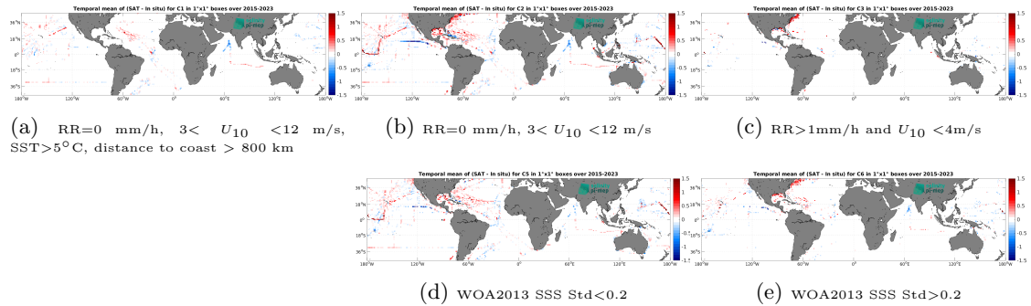
Figure 12: Temporal mean gridded over spatial boxes of size 1^\circ \times 1^\circ of \Delta SSS (SMAP SSS L3 v5 - Monthly (RSS) - TSG (SAMOS)) for 5 different subdatasets corresponding to:RR=0 mm/h, 3 < U_{10} < 12 m/s, SST >5^\circ C, distance to coast > 800 km (a), RR=0 mm/h, 3 < U_{10} < 12 m/s (b), RR >1 mm/h and U_{10} < 4 m/s (c), WOA2013 SSS Std <0.2 (d), WOA2013 SSS Std >0.2 (e).
