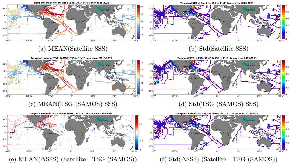
Figure 6: Temporal mean (left) and Std (right) of SSS from SMAP SSS L3 v5 - Monthly (RSS) (top), TSG (SAMOS) (middle), and of \Delta SSS (Satellite - TSG (SAMOS)). Only match-up pairs are used to generate these maps.
