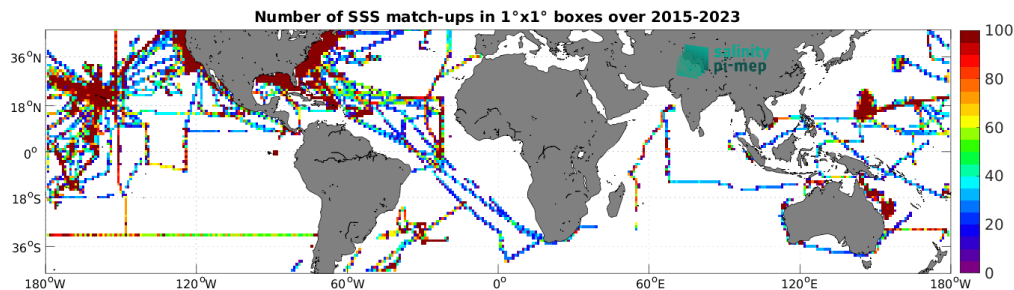
Figure 4: Number of SSS match-ups between TSG (SAMOS) SSS and the SMAP SSS L3 v5 - Monthly (RSS) SSS product for the Mid-Low Latitudes 45N-45S Pi-MEP region over 1^\circ \times 1^\circ boxes and for the full satellite product period.
