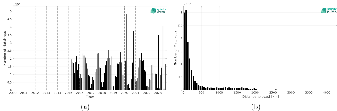
Figure 1: Number of match-ups between TSG (SAMOS) and SMAP SSS L3 v5 - Monthly (RSS) SSS as a function of time (a) and as function of the distance to coast (b) over the Mid-Low Latitudes 45N-45S Pi-MEP region and for the full satellite product period.
