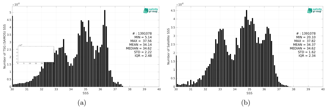
Figure 2: Histograms of SSS from TSG (SAMOS) (a) and SMAP SSS L3 v5 - Monthly (RSS) (b) considering all match-up pairs per bins of 0.1 over the Mid-Low Latitudes 45N-45S Pi-MEP region and for the full satellite product period.
