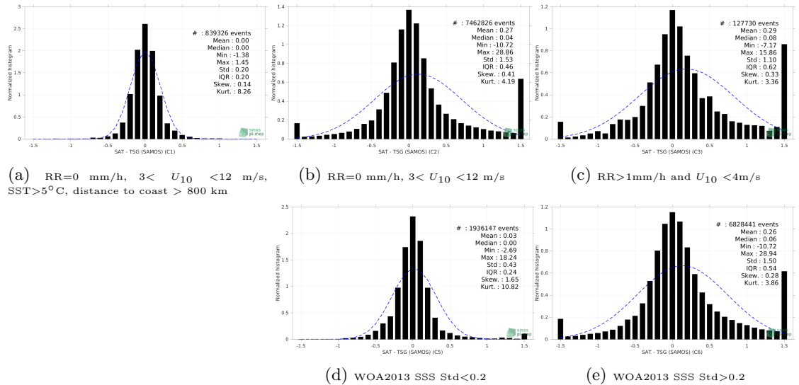
Figure 13: Normalized histogram of \Delta SSS (SMAP SSS L3 v5 - Monthly (RSS) - TSG (SAMOS)) for 5 different subdatasets corresponding to: RR=0 mm/h, 3 < U_{10} < 12 m/s, SST >5^\circ\text{C} , distance to coast > 800 km (a), RR=0 mm/h, 3 < U_{10} < 12 m/s (b), RR >1 mm/h and U_{10} < 4 m/s (c), WOA2013 SSS Std <0.2 (d), WOA2013 SSS Std >0.2 (e).
