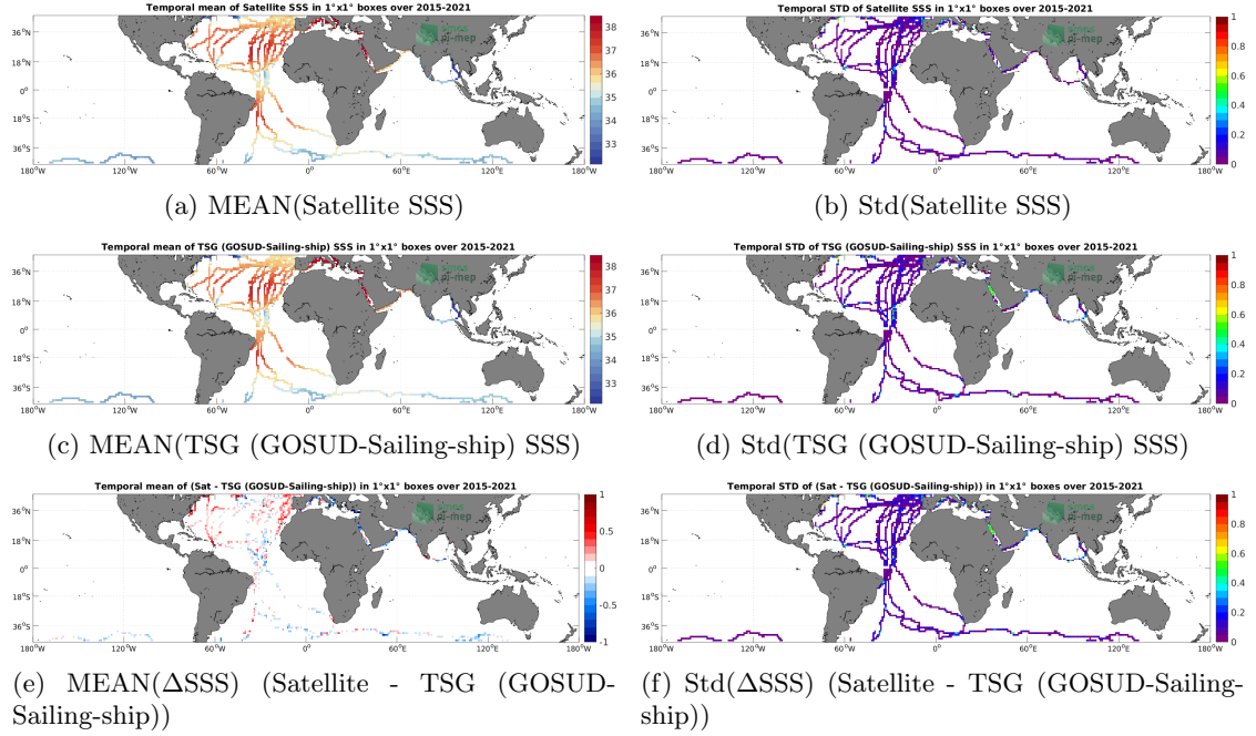
Figure 6: Temporal mean (left) and Std (right) of SSS from SMAP SSS L3 v5 - Monthly (RSS) (top), TSG (GOSUD-Sailing-ship) (middle), and of \Delta SSS (Satellite - TSG (GOSUD-Sailing-ship)). Only match-up pairs are used to generate these maps.
