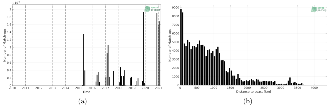
Figure 1: Number of match-ups between TSG (GOSUD-Sailing-ship) and SMAP SSS L3 v5 - Monthly (RSS) SSS as a function of time (a) and as function of the distance to coast (b) over the Mid-Low Latitudes 45N-45S Pi-MEP region and for the full satellite product period.
