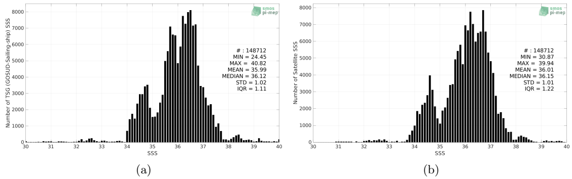
Figure 2: Histograms of SSS from TSG (GOSUD-Sailing-ship) (a) and SMAP SSS L3 v5 - Monthly (RSS) (b) considering all match-up pairs per bins of 0.1 over the Mid-Low Latitudes 45N-45S Pi-MEP region and for the full satellite product period.
