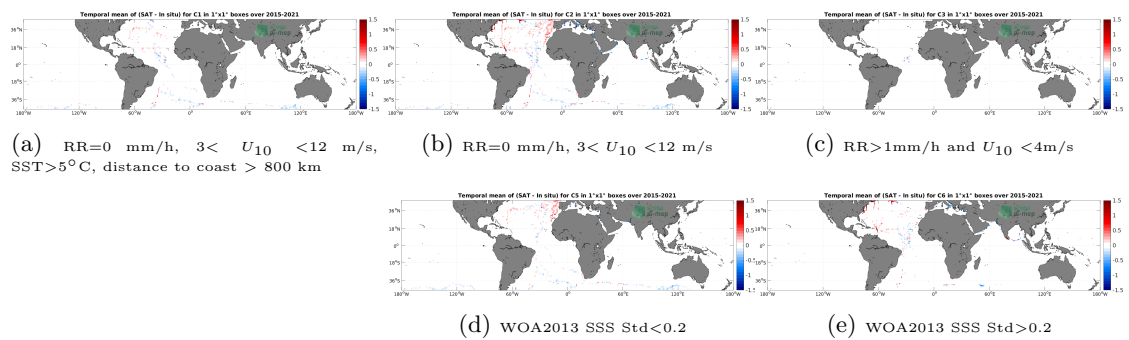
Figure 12: Temporal mean gridded over spatial boxes of size 1^\circ \times 1^\circ of \Delta SSS (SMAP SSS L3 v5 - Monthly (RSS) - TSG (GOSUD-Sailing-ship)) for 5 different subdatasets corresponding to:RR=0 mm/h, 3 < U_{10} < 12 m/s, SST>5°C, distance to coast > 800 km (a), RR=0 mm/h, 3 < U_{10} < 12 m/s (b), RR>1mm/h and U_{10} < 4 m/s (c), WOA2013 SSS Std<0.2 (d), WOA2013 SSS Std>0.2 (e).
