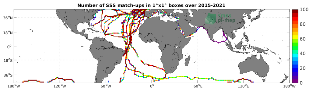
Figure 4: Number of SSS match-ups between TSG (GOSUD-Sailing-ship) SSS and the SMAP SSS L3 v5 - Monthly (RSS) SSS product for the Mid-Low Latitudes 45N-45S Pi-MEP region over 1^\circ \times 1^\circ boxes and for the full satellite product period.
