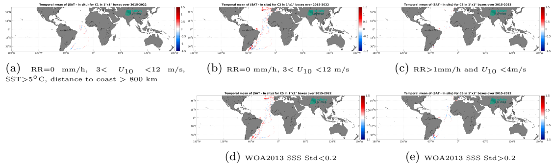
Figure 12: Temporal mean gridded over spatial boxes of size 1^\circ \times 1^\circ of \Delta SSS (SMAP SSS L3 v5 - Monthly (RSS) - TSG (CSIC-UTM)) for 5 different subdatasets corresponding to:RR=0 mm/h, 3 < U_{10} < 12 m/s, SST >5^\circ\text{C} , distance to coast > 800 km (a), RR=0 mm/h, 3 < U_{10} < 12 m/s (b), RR >1 mm/h and U_{10} < 4 m/s (c), WOA2013 SSS Std <0.2 (d), WOA2013 SSS Std >0.2 (e).
