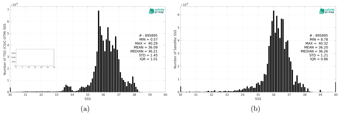
Figure 2: Histograms of SSS from TSG (CSIC-UTM) (a) and SMAP SSS L3 v5 - Monthly (RSS) (b) considering all match-up pairs per bins of 0.1 over the Mid-Low Latitudes 45N-45S Pi-MEP region and for the full satellite product period.
