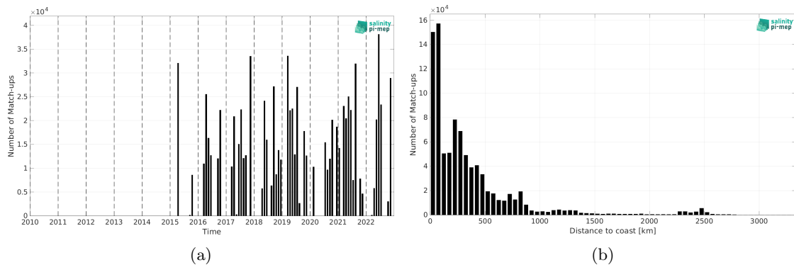
Figure 1: Number of match-ups between TSG (CSIC-UTM) and SMAP SSS L3 v5 - Monthly (RSS) SSS as a function of time (a) and as function of the distance to coast (b) over the Mid-Low Latitudes 45N-45S Pi-MEP region and for the full satellite product period.
