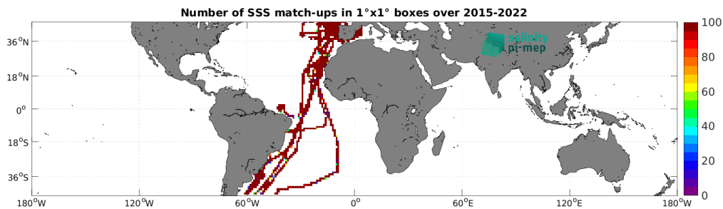
Figure 4: Number of SSS match-ups between TSG (CSIC-UTM) SSS and the SMAP SSS L3 v5 - Monthly (RSS) SSS product for the Mid-Low Latitudes 45N-45S Pi-MEP region over 1^\circ \times 1^\circ boxes and for the full satellite product period.
