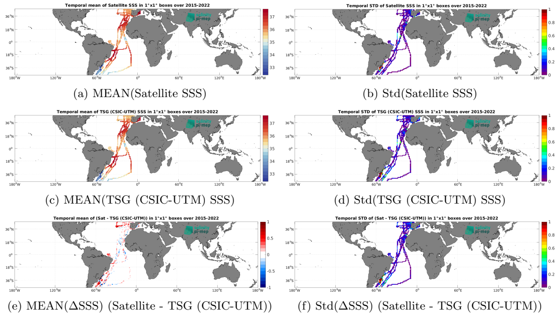
Figure 6: Temporal mean (left) and Std (right) of SSS from SMAP SSS L3 v5 - Monthly (RSS) (top), TSG (CSIC-UTM) (middle), and of \Delta SSS (Satellite - TSG (CSIC-UTM)). Only match-up pairs are used to generate these maps.
