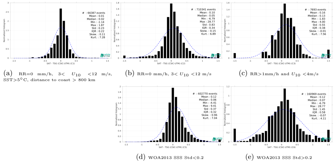
Figure 13: Normalized histogram of \Delta SSS (SMAP SSS L3 v5 - Monthly (RSS) - TSG (CSIC-UTM)) for 5 different subdatasets corresponding to: RR=0 mm/h, 3 < U_{10} < 12 m/s, SST >5^\circ\text{C} , distance to coast > 800 km (a), RR=0 mm/h, 3 < U_{10} < 12 m/s (b), RR >1 mm/h and U_{10} < 4 m/s (c), WOA2013 SSS Std <0.2 (d), WOA2013 SSS Std >0.2 (e).
