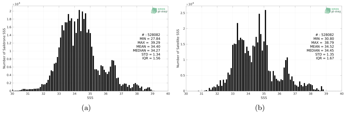
Figure 2: Histograms of SSS from Saildrone (a) and SMAP SSS L3 v5 - Monthly (RSS) (b) considering all match-up pairs per bins of 0.1 over the Mid-Low Latitudes 45N-45S Pi-MEP region and for the full satellite product period.
