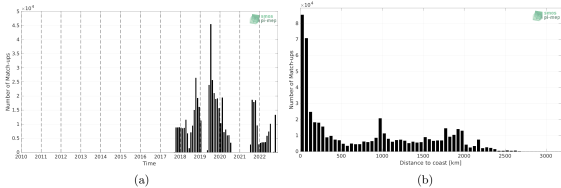
Figure 1: Number of match-ups between Saildrone and SMAP SSS L3 v5 - Monthly (RSS) SSS as a function of time (a) and as function of the distance to coast (b) over the Mid-Low Latitudes 45N-45S Pi-MEP region and for the full satellite product period.
