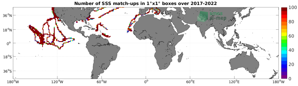
Figure 4: Number of SSS match-ups between Saildrone SSS and the SMAP SSS L3 v5 - Monthly (RSS) SSS product for the Mid-Low Latitudes 45N-45S Pi-MEP region over 1^\circ \times 1^\circ boxes and for the full satellite product period.
