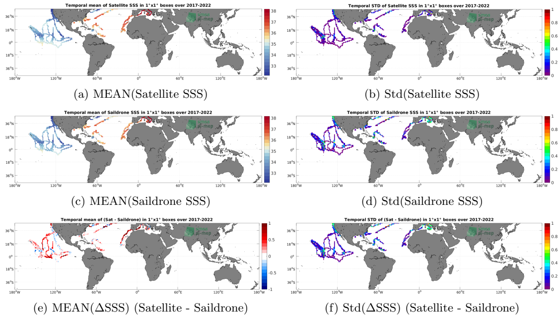
Figure 6: Temporal mean (left) and Std (right) of SSS from SMAP SSS L3 v5 - Monthly (RSS) (top), Saildrone (middle), and of \Delta SSS (Satellite - Saildrone). Only match-up pairs are used to generate these maps.
