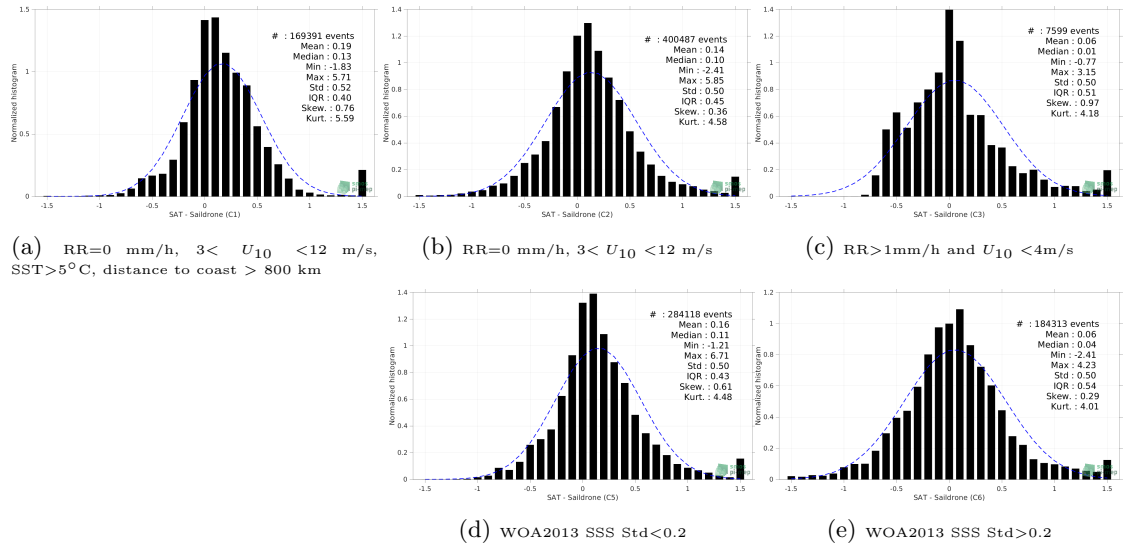
Figure 13: Normalized histogram of \Delta SSS (SMAP SSS L3 v5 - Monthly (RSS) - Saildrone) for 5 different subdatasets corresponding to: RR=0 mm/h, 3 < U_{10} < 12 m/s, SST >5^\circ\text{C} , distance to coast > 800 km (a), RR=0 mm/h, 3 < U_{10} < 12 m/s (b), RR >1 mm/h and U_{10} < 4 m/s (c), WOA2013 SSS Std <0.2 (d), WOA2013 SSS Std >0.2 (e).
