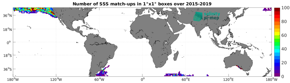
Figure 4: Number of SSS match-ups between Marine mammals SSS and the SMAP SSS L3 v5 - Monthly (RSS) SSS product for the Mid-Low Latitudes 45N-45S Pi-MEP region over 1^\circ \times 1^\circ boxes and for the full satellite product period.
