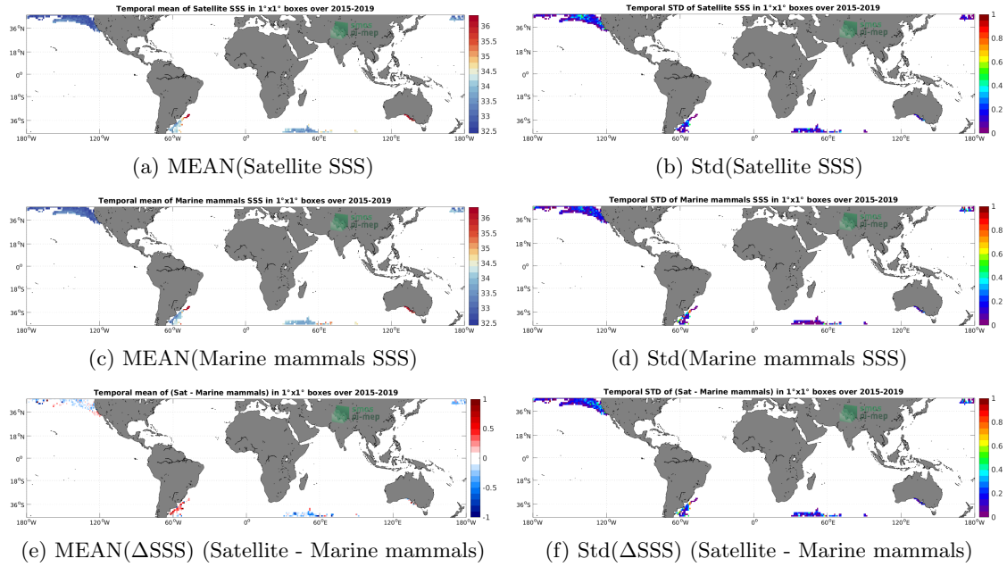
Figure 6: Temporal mean (left) and Std (right) of SSS from SMAP SSS L3 v5 - Monthly (RSS) (top), Marine mammals (middle), and of \Delta SSS (Satellite - Marine mammals). Only match-up pairs are used to generate these maps.
