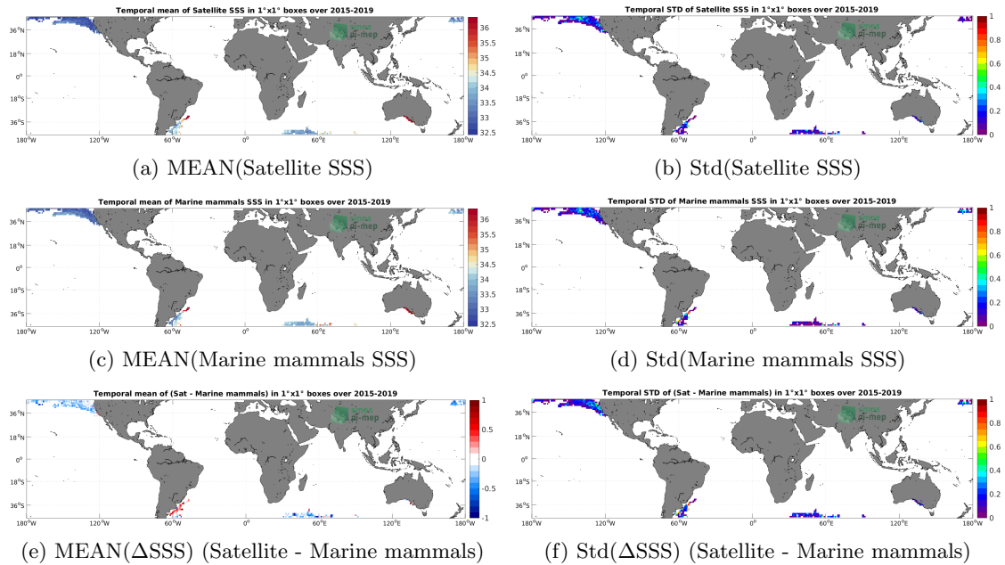
Figure 6: Temporal mean (left) and Std (right) of SSS from SMAP SSS L3 v5 - Monthly (RSS) (top), Marine mammals (middle), and of \Delta SSS (Satellite - Marine mammals). Only match-up pairs are used to generate these maps.
