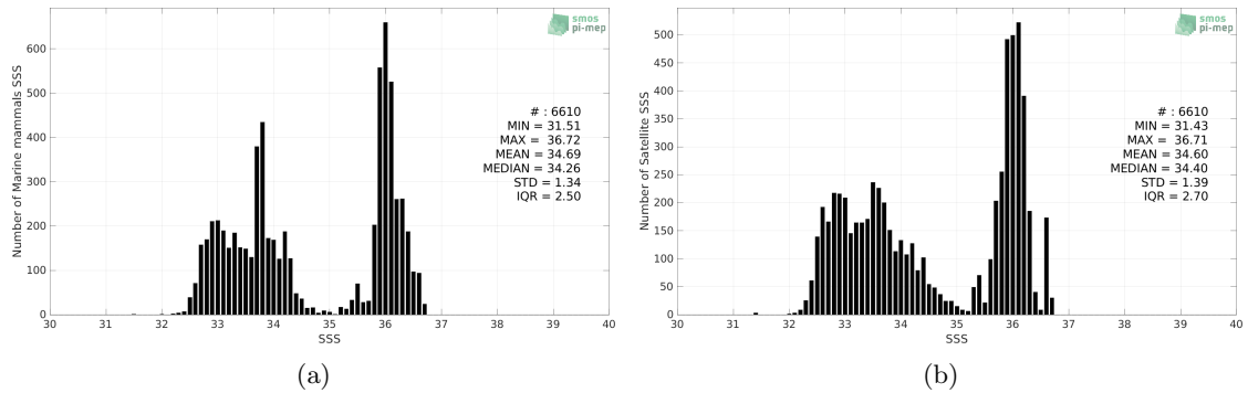
Figure 2: Histograms of SSS from Marine mammals (a) and SMAP SSS L3 v5 - Monthly (RSS) (b) considering all match-up pairs per bins of 0.1 over the Mid-Low Latitudes 45N-45S Pi-MEP region and for the full satellite product period.
