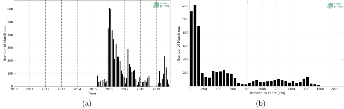
Figure 1: Number of match-ups between Marine mammals and SMAP SSS L3 v5 - Monthly (RSS) SSS as a function of time (a) and as function of the distance to coast (b) over the Mid-Low Latitudes 45N-45S Pi-MEP region and for the full satellite product period.
