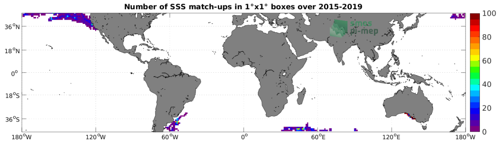
Figure 4: Number of SSS match-ups between Marine mammals SSS and the SMAP SSS L3 v5 - Monthly (RSS) SSS product for the Mid-Low Latitudes 45N-45S Pi-MEP region over 1^{\circ} \times 1^{\circ} boxes and for the full satellite product period.
