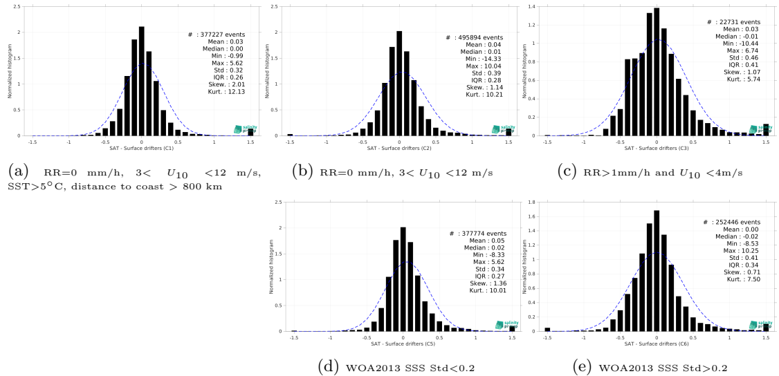
Figure 12: Normalized histogram of \Delta SSS (SMAP SSS L3 v5 - Monthly (RSS) - Surface drifters) for 5 different subdatasets corresponding to: RR=0 mm/h, 3 < U_{10} < 12 m/s, SST >5^\circ C, distance to coast > 800 km (a), RR=0 mm/h, 3 < U_{10} < 12 m/s (b), RR >1 mm/h and U_{10} < 4 m/s (c), WOA2013 SSS Std <0.2 (d), WOA2013 SSS Std >0.2 (e).
