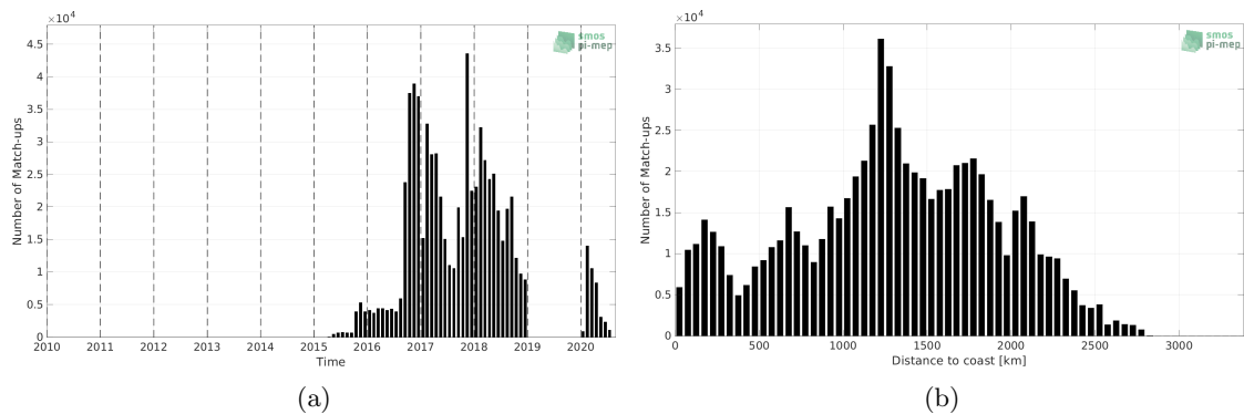
Figure 1: Number of match-ups between Surface drifters and SMAP SSS L3 v5 - Monthly (RSS) SSS as a function of time (a) and as function of the distance to coast (b) over the Mid-Low Latitudes 45N-45S Pi-MEP region and for the full satellite product period.
