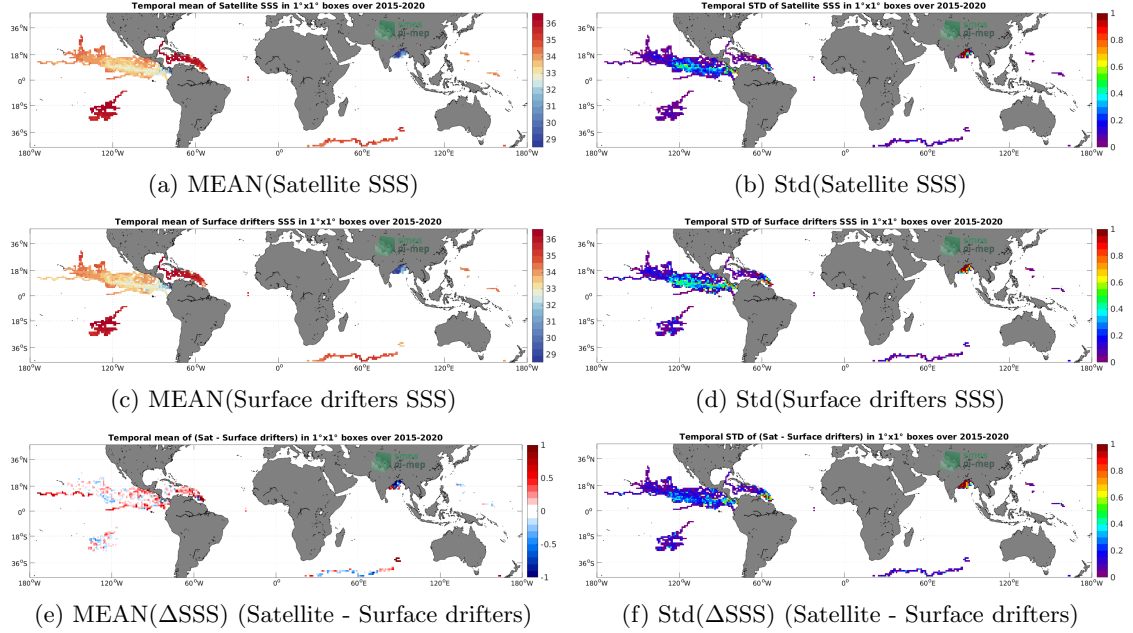
Figure 5: Temporal mean (left) and Std (right) of SSS from SMAP SSS L3 v5 - Monthly (RSS) (top), Surface drifters (middle), and of \Delta\text{SSS} (Satellite - Surface drifters). Only match-up pairs are used to generate these maps.
