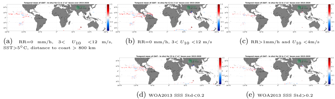
Figure 11: Temporal mean gridded over spatial boxes of size 1^\circ \times 1^\circ of \Delta SSS (SMAP SSS L3 v5 - Monthly (RSS) - Surface drifters) for 5 different subdatasets corresponding to:RR=0 mm/h, 3 < U_{10} < 12 m/s, SST >5^\circ\text{C} , distance to coast > 800 km (a), RR=0 mm/h, 3 < U_{10} < 12 m/s (b), RR >1 mm/h and U_{10} < 4 m/s (c), WOA2013 SSS Std <0.2 (d), WOA2013 SSS Std >0.2 (e).
