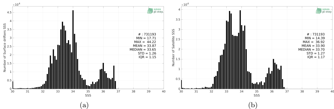
Figure 2: Histograms of SSS from Surface drifters (a) and SMAP SSS L3 v5 - Monthly (RSS) (b) considering all match-up pairs per bins of 0.1 over the Mid-Low Latitudes 45N-45S Pi-MEP region and for the full satellite product period.
