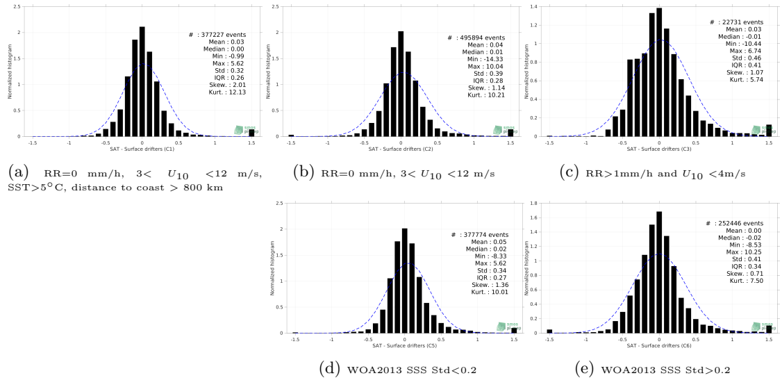
Figure 12: Normalized histogram of \Delta SSS (SMAP SSS L3 v5 - Monthly (RSS) - Surface drifters) for 5 different subdatasets corresponding to: RR=0 mm/h, 3 < U_{10} < 12 m/s, SST >5^\circ\text{C} , distance to coast > 800 km (a), RR=0 mm/h, 3 < U_{10} < 12 m/s (b), RR >1 mm/h and U_{10} < 4 m/s (c), WOA2013 SSS Std <0.2 (d), WOA2013 SSS Std >0.2 (e).
