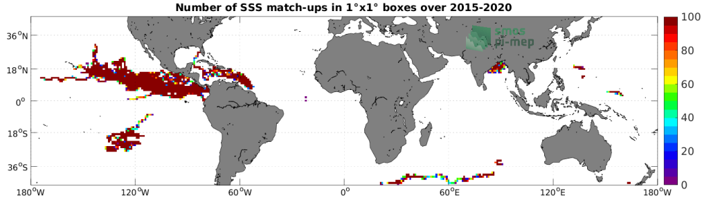
Figure 3: Number of SSS match-ups between Surface drifters SSS and the SMAP SSS L3 v5 - Monthly (RSS) SSS product for the Mid-Low Latitudes 45N-45S Pi-MEP region over 1^\circ \times 1^\circ boxes and for the full satellite product period.
