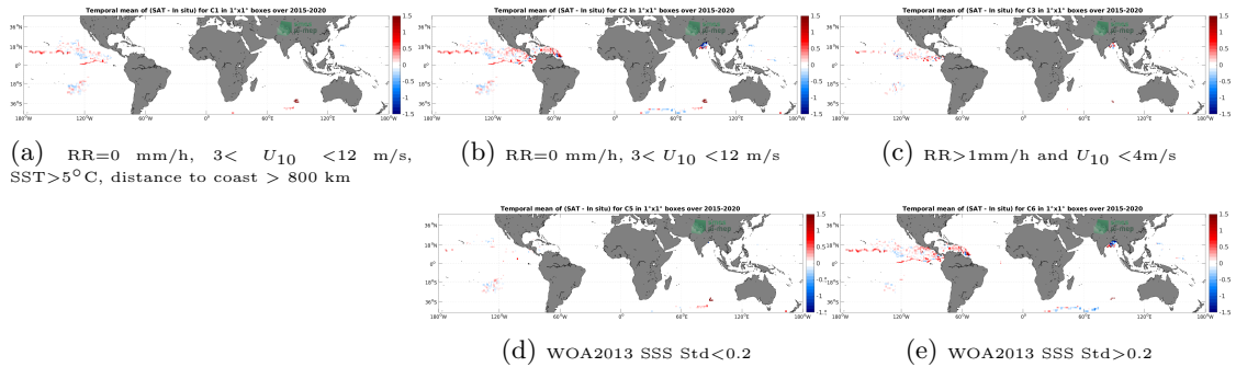
Figure 11: Temporal mean gridded over spatial boxes of size 1^\circ \times 1^\circ of \Delta SSS (SMAP SSS L3 v5 - Monthly (RSS) - Surface drifters) for 5 different subdatasets corresponding to: RR=0 mm/h, 3 < U_{10} < 12 m/s, SST >5^\circ\text{C} , distance to coast > 800 km (a), RR=0 mm/h, 3 < U_{10} < 12 m/s (b), RR >1 mm/h and U_{10} < 4 m/s (c), WOA2013 SSS Std <0.2 (d), WOA2013 SSS Std >0.2 (e).
