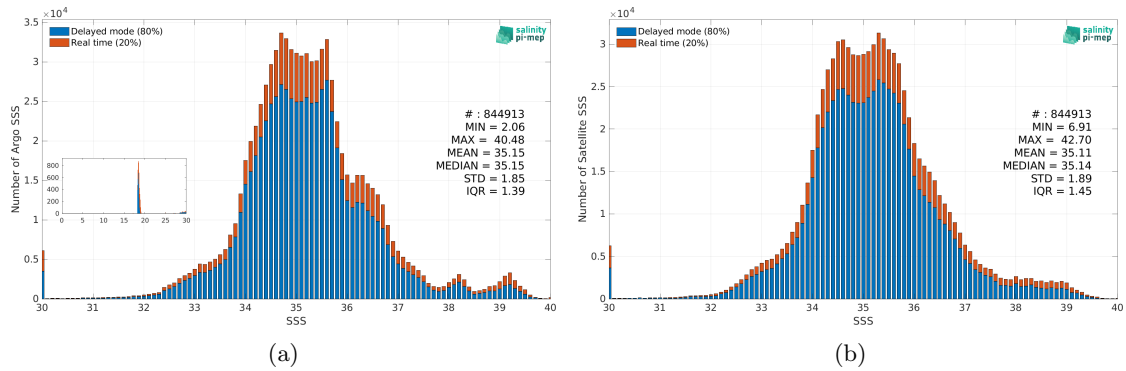
Figure 2: Histograms of SSS from Argo (a) and SMAP SSS L3 v5 - Monthly (RSS) (b) considering all match-up pairs per bins of 0.1 over the Mid-Low Latitudes 45N-45S Pi-MEP region and for the full satellite product period.
