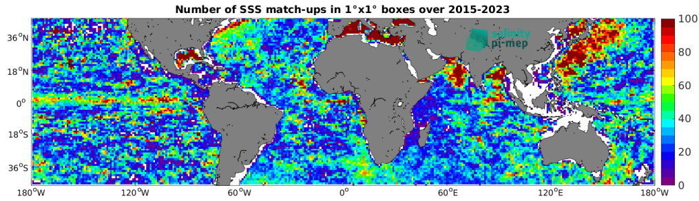
Figure 4: Number of SSS match-ups between Argo SSS and the SMAP SSS L3 v5 - Monthly (RSS) SSS product for the Mid-Low Latitudes 45N-45S Pi-MEP region over 1^\circ \times 1^\circ boxes and for the full satellite product period.
