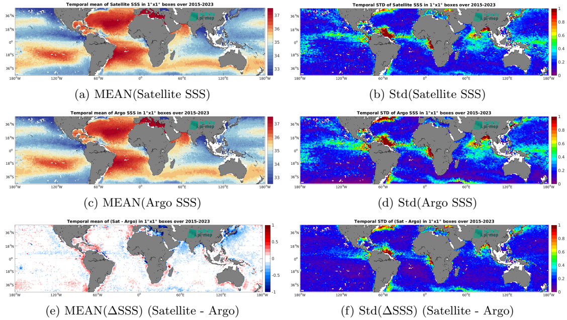
Figure 6: Temporal mean (left) and Std (right) of SSS from SMAP SSS L3 v5 - Monthly (RSS) (top), Argo (middle), and of \Delta SSS (Satellite - Argo). Only match-up pairs are used to generate these maps.
