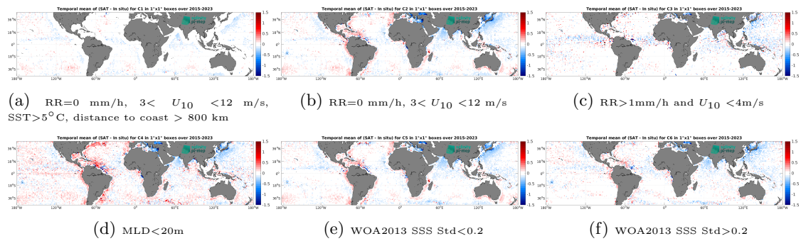
Figure 12: Temporal mean gridded over spatial boxes of size 1^\circ \times 1^\circ of \Delta SSS (SMAP SSS L3 v5 - Monthly (RSS) - Argo) for 6 different subdatasets corresponding to:RR=0 mm/h, 3 < U_{10} < 12 m/s, SST >5^\circ C, distance to coast > 800 km (a), RR=0 mm/h, 3 < U_{10} < 12 m/s (b), RR >1 mm/h and U_{10} < 4 m/s (c),MLD <20 m (d),WOA2013 SSS Std <0.2 (e),WOA2013 SSS Std >0.2 (f).
