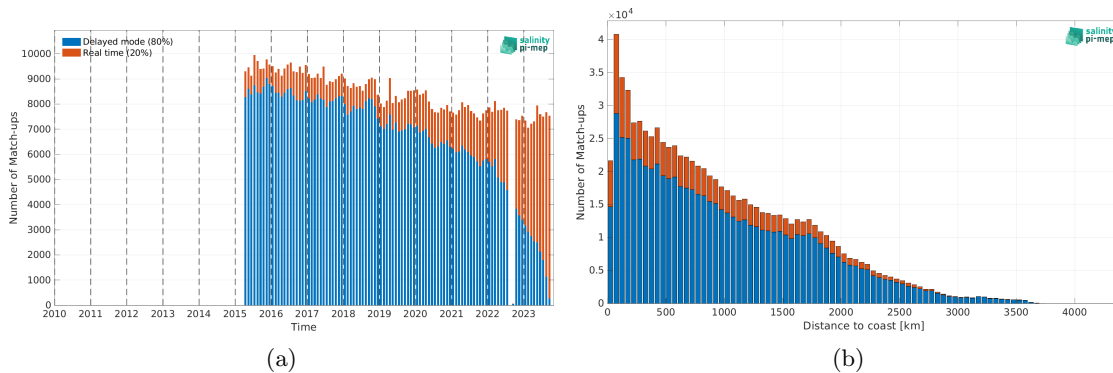
Figure 1: Number of match-ups between Argo and SMAP SSS L3 v5 - Monthly (RSS) SSS as a function of time (a) and as function of the distance to coast (b) over the Mid-Low Latitudes 45N-45S Pi-MEP region and for the full satellite product period.
