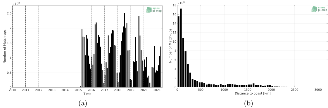
Figure 1: Number of match-ups between TSG (SAMOS) and SMAP SSS L3 v4 - 8-Day running (RSS) SSS as a function of time (a) and as function of the distance to coast (b) over the Mid-Low Latitudes 45N-45S Pi-MEP region and for the full satellite product period.
