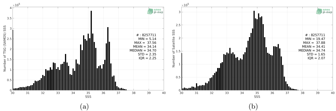
Figure 2: Histograms of SSS from TSG (SAMOS) (a) and SMAP SSS L3 v4 - 8-Day running (RSS) (b) considering all match-up pairs per bins of 0.1 over the Mid-Low Latitudes 45N-45S Pi-MEP region and for the full satellite product period.
