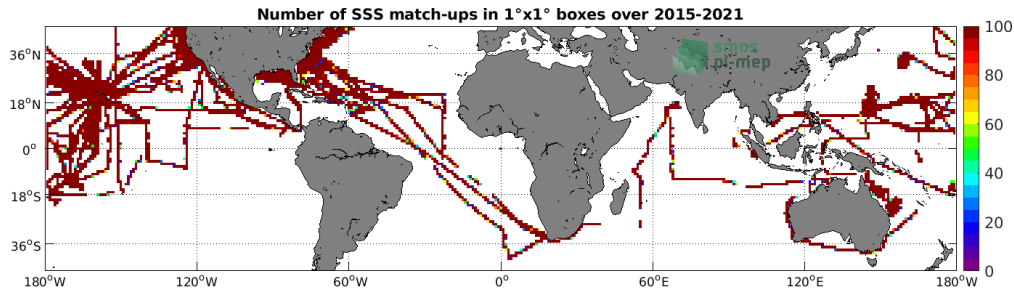
Figure 4: Number of SSS match-ups between TSG (SAMOS) SSS and the SMAP SSS L3 v4 - 8-Day running (RSS) SSS product for the Mid-Low Latitudes 45N-45S Pi-MEP region over 1^\circ \times 1^\circ boxes and for the full satellite product period.
