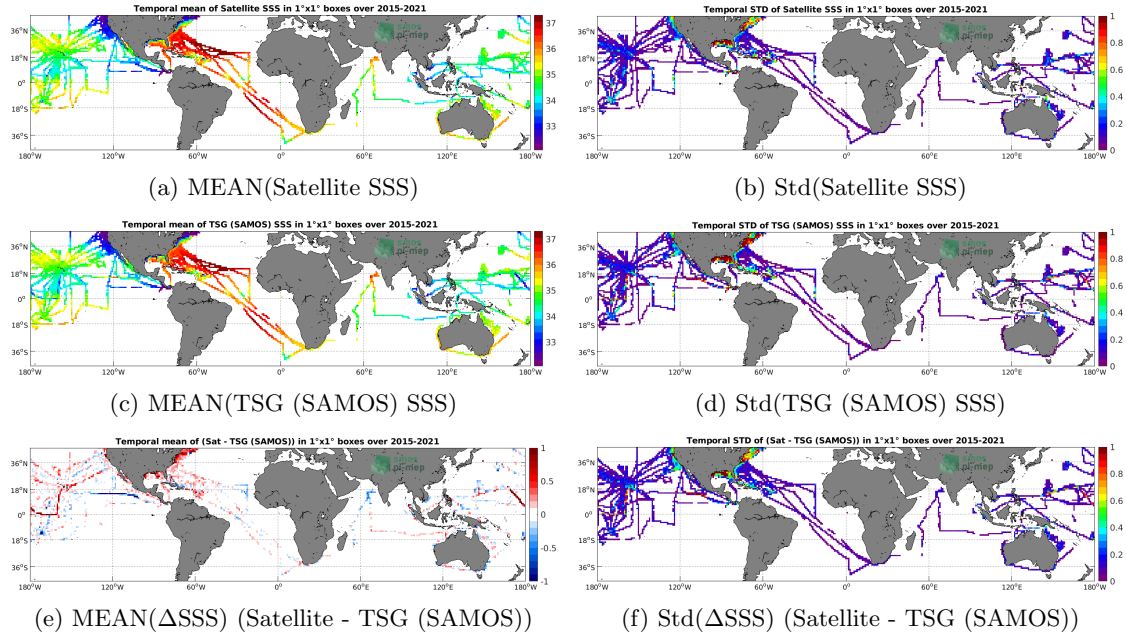
Figure 6: Temporal mean (left) and Std (right) of SSS from SMAP SSS L3 v4 - 8-Day running (RSS) (top), TSG (SAMOS) (middle), and of \Delta SSS (Satellite - TSG (SAMOS)). Only match-up pairs are used to generate these maps.
