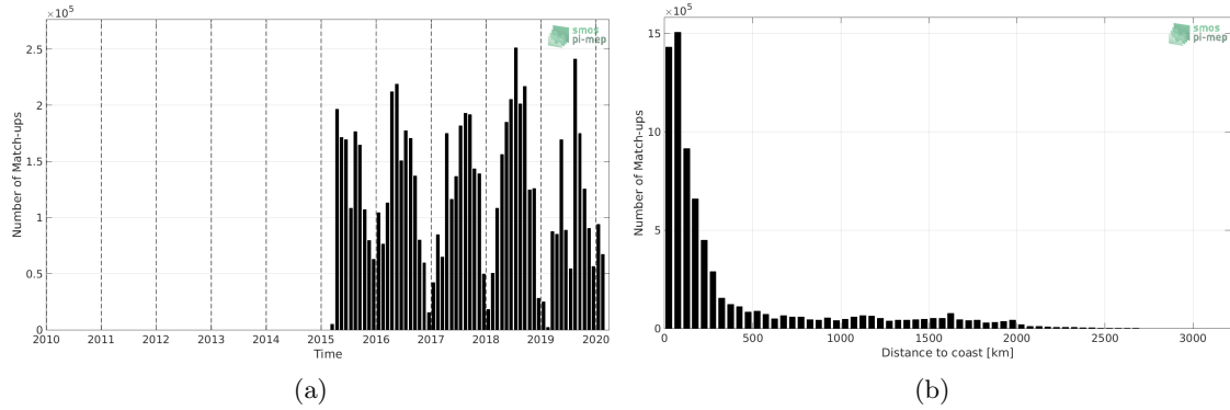
Figure 1: Number of match-ups between TSG-SAMOS and SMAP-L3-RSS-V4-8DAY-RUNNING SSS as a function of time (a) and as function of the distance to coast (b) over the Mid-Low Latitudes 45N-45S Pi-MEP region and for the full satellite product period.
