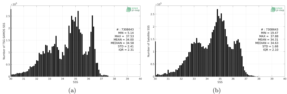
Figure 2: Histograms of SSS from TSG-SAMOS (a) and SMAP-L3-RSS-V4-8DAY-RUNNING (b) considering all match-up pairs per bins of 0.1 over the Mid-Low Latitudes 45N-45S Pi-MEP region and for the full satellite product period.
