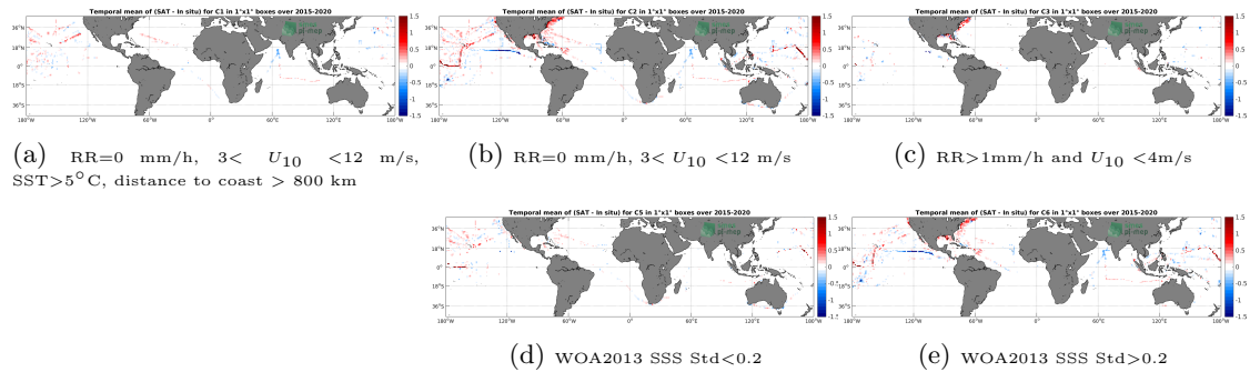
Figure 12: Temporal mean gridded over spatial boxes of size 1^\circ \times 1^\circ of \Delta SSS (SMAP-L3-RSS-V4-8DAY-RUNNING - TSG-SAMOS) for 5 different subdatasets corresponding to:RR=0 mm/h, 3 < U_{10} < 12 m/s, SST >5^\circ\text{C} , distance to coast > 800 km (a), RR=0 mm/h, 3 < U_{10} < 12 m/s (b), RR >1 mm/h and U_{10} < 4 m/s (c), WOA2013 SSS Std <0.2 (d), WOA2013 SSS Std >0.2 (e).
