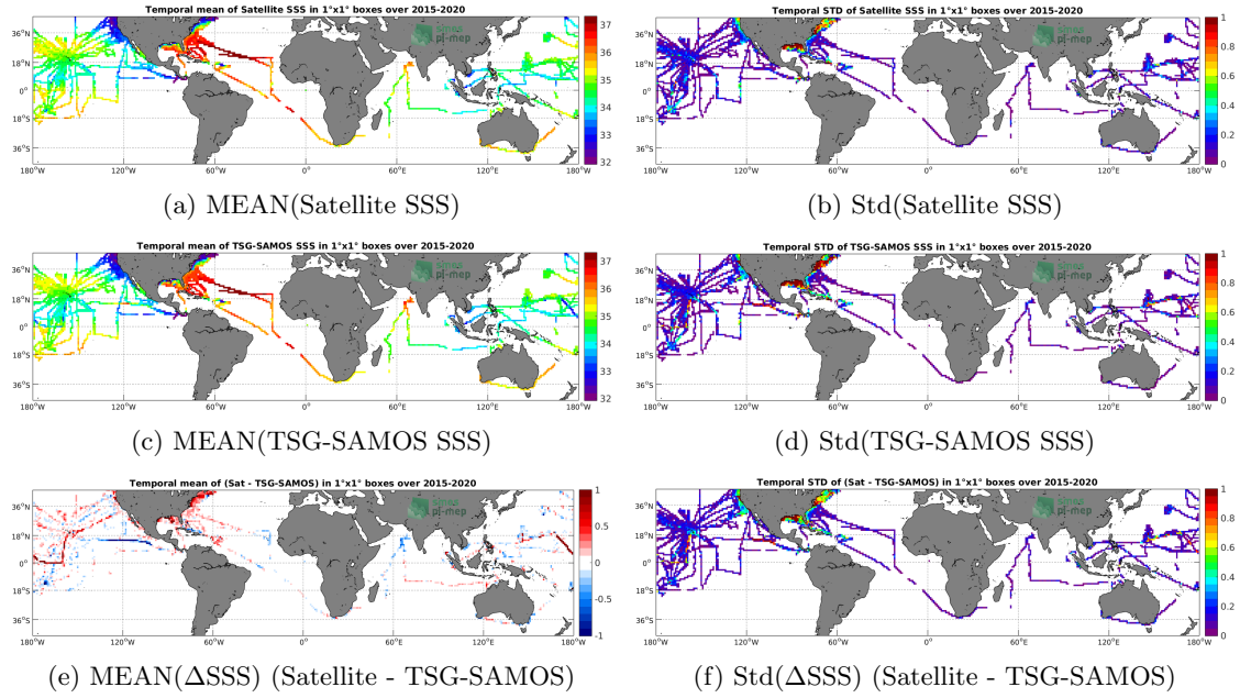
Figure 6: Temporal mean (left) and Std (right) of SSS from SMAP-L3-RSS-V4-8DAY-RUNNING (top), TSG-SAMOS (middle), and of \Delta SSS (Satellite - TSG-SAMOS). Only match-up pairs are used to generate these maps.
