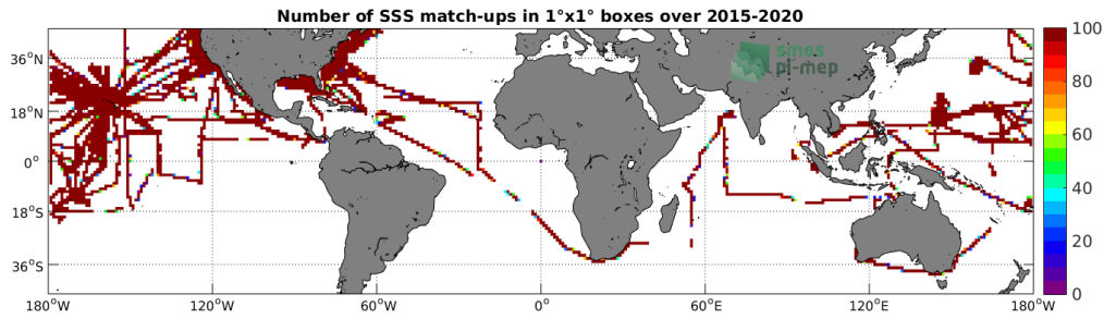
Figure 4: Number of SSS match-ups between TSG-SAMOS SSS and the SMAP-L3-RSS-V4-8DAY-RUNNING SSS product for the Mid-Low Latitudes 45N-45S Pi-MEP region over 1^\circ \times 1^\circ boxes and for the full satellite product period.
