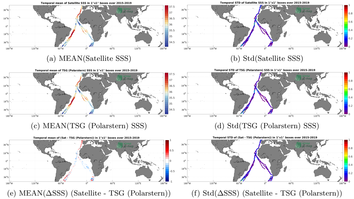
Figure 6: Temporal mean (left) and Std (right) of SSS from SMAP SSS L3 v4 - 8-Day running (RSS) (top), TSG (Polarstern) (middle), and of \Delta SSS (Satellite - TSG (Polarstern)). Only match-up pairs are used to generate these maps.
