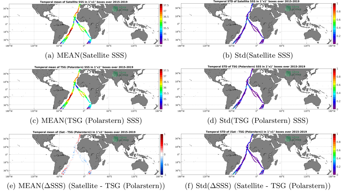
Figure 6: Temporal mean (left) and Std (right) of SSS from SMAP SSS L3 v4 - 8-Day running (RSS) (top), TSG (Polarstern) (middle), and of \Delta SSS (Satellite - TSG (Polarstern)). Only match-up pairs are used to generate these maps.
