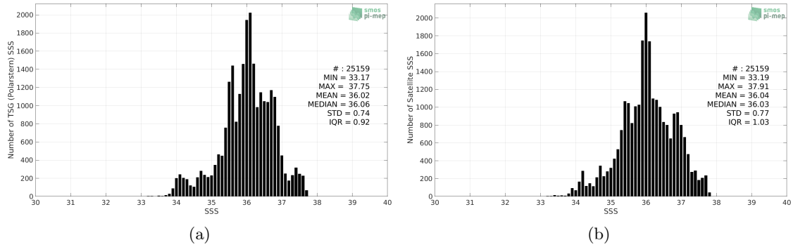
Figure 2: Histograms of SSS from TSG (Polarstern) (a) and SMAP SSS L3 v4 - 8-Day running (RSS) (b) considering all match-up pairs per bins of 0.1 over the Mid-Low Latitudes 45N-45S Pi-MEP region and for the full satellite product period.
