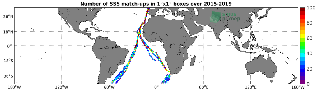
Figure 4: Number of SSS match-ups between TSG (Polarstern) SSS and the SMAP SSS L3 v4 - 8-Day running (RSS) SSS product for the Mid-Low Latitudes 45N-45S Pi-MEP region over 1^\circ \times 1^\circ boxes and for the full satellite product period.
