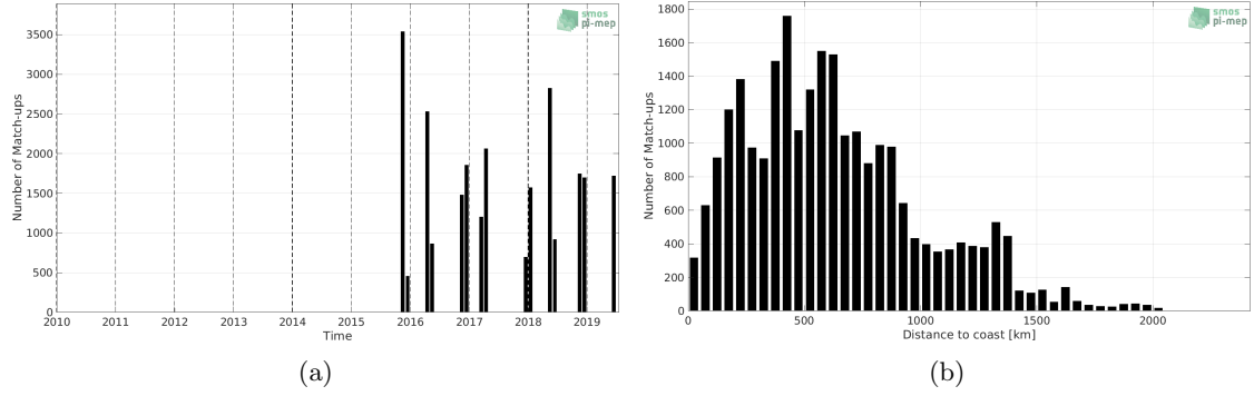
Figure 1: Number of match-ups between TSG (Polarstern) and SMAP SSS L3 v4 - 8-Day running (RSS) SSS as a function of time (a) and as function of the distance to coast (b) over the Mid-Low Latitudes 45N-45S Pi-MEP region and for the full satellite product period.
