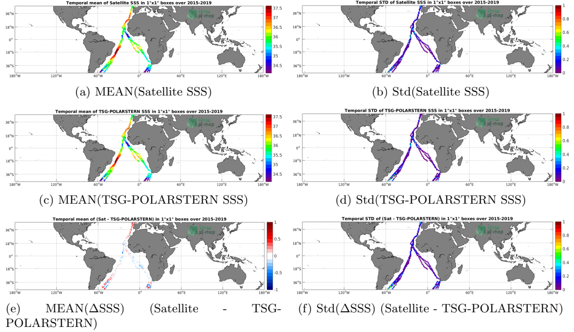
Figure 6: Temporal mean (left) and Std (right) of SSS from SMAP-L3-RSS-V4-8DAY-RUNNING (top), TSG-POLARSTERN (middle), and of \Delta SSS (Satellite - TSG-POLARSTERN). Only match-up pairs are used to generate these maps.
