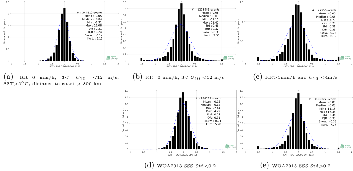
Figure 13: Normalized histogram of \Delta\text{SSS} (SMAP SSS L3 v4 - 8-Day running (RSS) - TSG (LEGOS-DM)) for 5 different subdatasets corresponding to: RR=0 mm/h, 3 < U_{10} < 12 m/s, SST>5°C, distance to coast > 800 km (a), RR=0 mm/h, 3 < U_{10} < 12 m/s (b), RR>1mm/h and U_{10} < 4 m/s (c), WOA2013 SSS Std<0.2 (d), WOA2013 SSS Std>0.2 (e).
