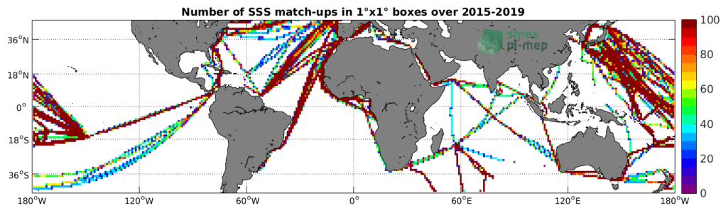
Figure 4: Number of SSS match-ups between TSG-LEGOS-DM SSS and the SMAP-L3-RSS-V4-8DAY-RUNNING SSS product for the Mid-Low Latitudes 45N-45S Pi-MEP region over 1^\circ \times 1^\circ boxes and for the full satellite product period.
