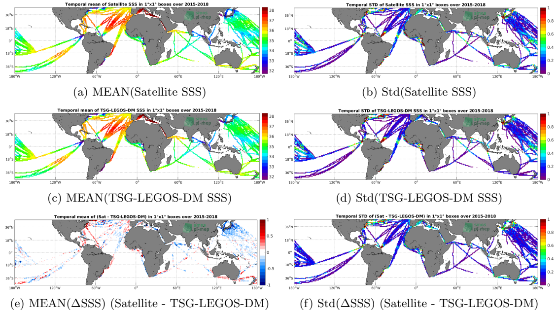
Figure 6: Temporal mean (left) and Std (right) of SSS from SMAP-L3-RSS-V4-8DAY-RUNNING (top), TSG-LEGOS-DM (middle), and of \Delta SSS (Satellite - TSG-LEGOS-DM). Only match-up pairs are used to generate these maps.
