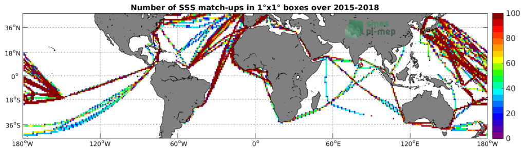
Figure 4: Number of SSS match-ups between TSG-LEGOS-DM SSS and the SMAP-L3-RSS-V4-8DAY-RUNNING SSS product for the Mid-Low Latitudes 45N-45S Pi-MEP region over 1°x1° boxes and for the full satellite product period.
