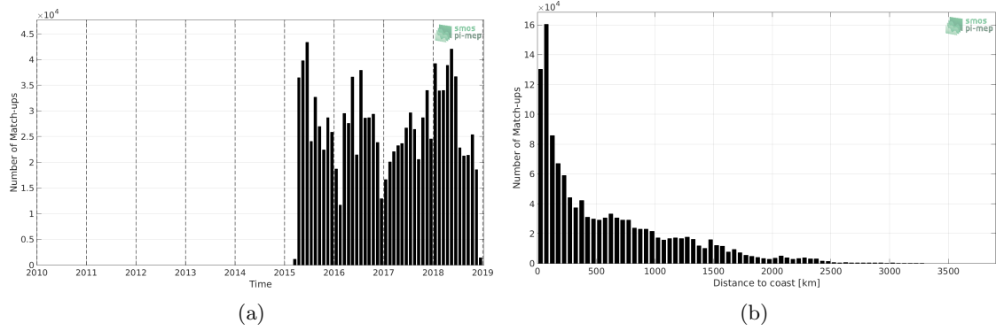
Figure 1: Number of match-ups between TSG-LEGOS-DM and SMAP-L3-RSS-V4-8DAY-RUNNING SSS as a function of time (a) and as function of the distance to coast (b) over the Mid-Low Latitudes 45N-45S Pi-MEP region and for the full satellite product period.
