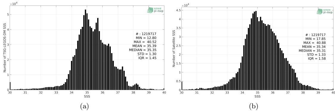
Figure 2: Histograms of SSS from TSG-LEGOS-DM (a) and SMAP-L3-RSS-V4-8DAY-RUNNING (b) considering all match-up pairs per bins of 0.1 over the Mid-Low Latitudes 45N-45S Pi-MEP region and for the full satellite product period.
