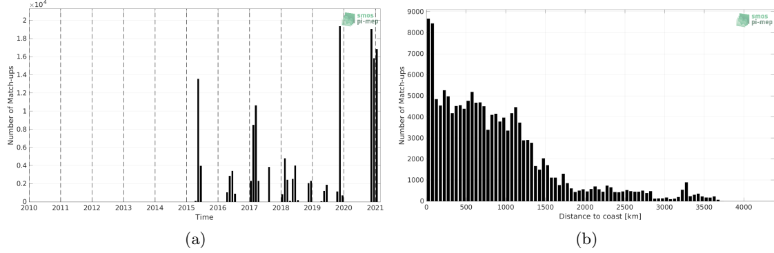
Figure 1: Number of match-ups between TSG (GOSUD-Sailing-ship) and SMAP SSS L3 v4 - 8-Day running (RSS) SSS as a function of time (a) and as function of the distance to coast (b) over the Mid-Low Latitudes 45N-45S Pi-MEP region and for the full satellite product period.
