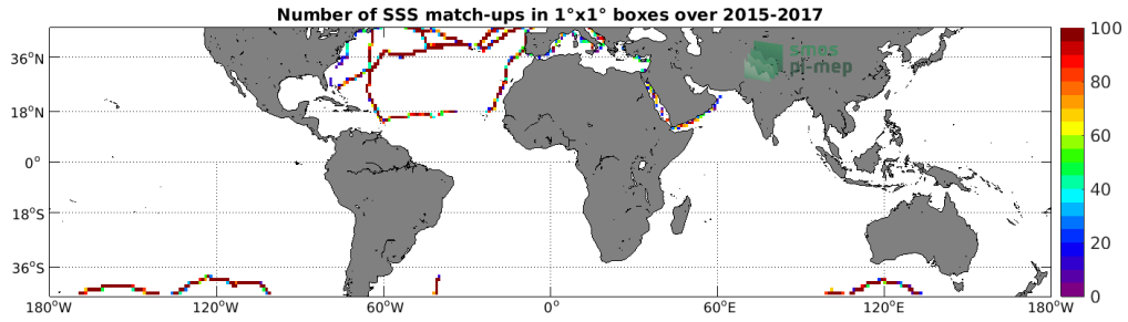
Figure 4: Number of SSS match-ups between TSG (GOSUD-Sailing-ship) SSS and the SMAP SSS L3 v4 - 8-Day running (RSS) SSS product for the Mid-Low Latitudes 45N-45S Pi-MEP region over 1^\circ \times 1^\circ boxes and for the full satellite product period.
