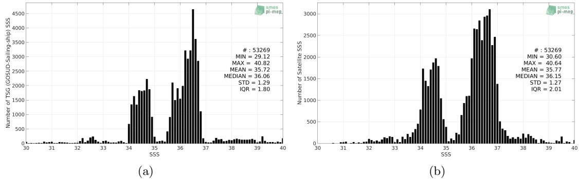
Figure 2: Histograms of SSS from TSG (GOSUD-Sailing-ship) (a) and SMAP SSS L3 v4 - 8-Day running (RSS) (b) considering all match-up pairs per bins of 0.1 over the Mid-Low Latitudes 45N-45S Pi-MEP region and for the full satellite product period.
