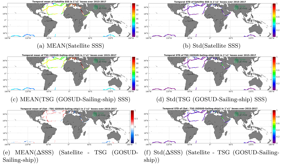
Figure 6: Temporal mean (left) and Std (right) of SSS from SMAP SSS L3 v4 - 8-Day running (RSS) (top), TSG (GOSUD-Sailing-ship) (middle), and of \Delta SSS (Satellite - TSG (GOSUD-Sailing-ship)). Only match-up pairs are used to generate these maps.
