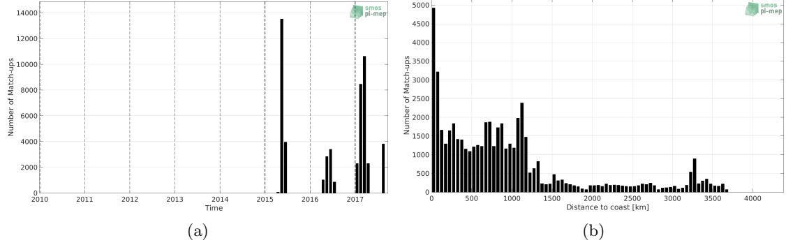
Figure 1: Number of match-ups between TSG (GOSUD-Sailing-ship) and SMAP SSS L3 v4 - 8-Day running (RSS) SSS as a function of time (a) and as function of the distance to coast (b) over the Mid-Low Latitudes 45N-45S Pi-MEP region and for the full satellite product period.
