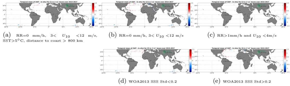
Figure 12: Temporal mean gridded over spatial boxes of size 1^\circ \times 1^\circ of \Delta SSS (SMAP SSS L3 v4 - 8-Day running (RSS) - TSG (GOSUD-Sailing-ship)) for 5 different subdatasets corresponding to: RR=0 mm/h, 3 < U_{10} < 12 m/s, SST > 5^\circ C , distance to coast > 800 km (a), RR=0 mm/h, 3 < U_{10} < 12 m/s (b), RR > 1 mm/h and U_{10} < 4 m/s (c), WOA2013 SSS Std < 0.2 (d), WOA2013 SSS Std > 0.2 (e).
