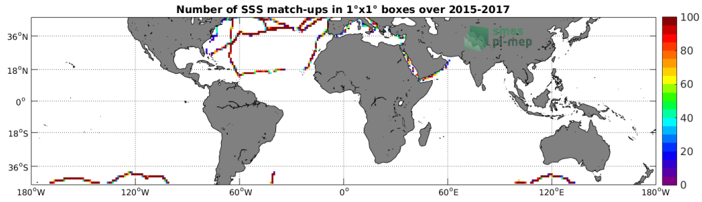
Figure 4: Number of SSS match-ups between TSG-GOSUD-Sailing-ship SSS and the SMAP-L3-RSS-V4-8DAY-RUNNING SSS product for the Mid-Low Latitudes 45N-45S Pi-MEP region over 1°x1° boxes and for the full satellite product period.
