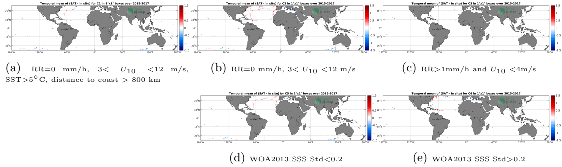
Figure 12: Temporal mean gridded over spatial boxes of size 1^\circ \times 1^\circ of \Delta SSS (SMAP-L3-RSS-V4-8DAY-RUNNING - TSG-GOSUD-Sailing-ship) for 5 different subdatasets corresponding to: RR=0 mm/h, 3 < U_{10} < 12 m/s, SST > 5^\circ C , distance to coast > 800 km (a), RR=0 mm/h, 3 < U_{10} < 12 m/s (b), RR > 1 mm/h and U_{10} < 4 m/s (c), WOA2013 SSS Std < 0.2 (d), WOA2013 SSS Std > 0.2 (e).
