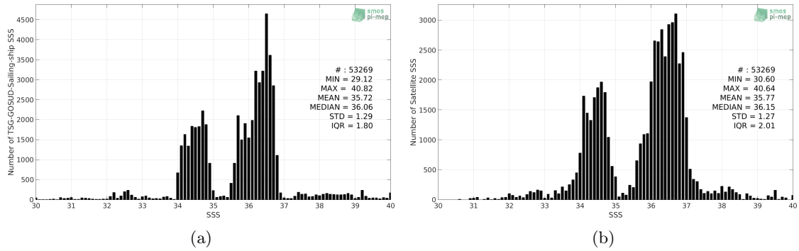
Figure 2: Histograms of SSS from TSG-GOSUD-Sailing-ship (a) and SMAP-L3-RSS-V4-8DAY-RUNNING (b) considering all match-up pairs per bins of 0.1 over the Mid-Low Latitudes 45N-45S Pi-MEP region and for the full satellite product period.
