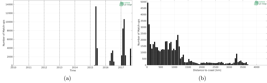
Figure 1: Number of match-ups between TSG-GOSUD-Sailing-ship and SMAP-L3-RSS-V4-8DAY-RUNNING SSS as a function of time (a) and as function of the distance to coast (b) over the Mid-Low Latitudes 45N-45S Pi-MEP region and for the full satellite product period.
