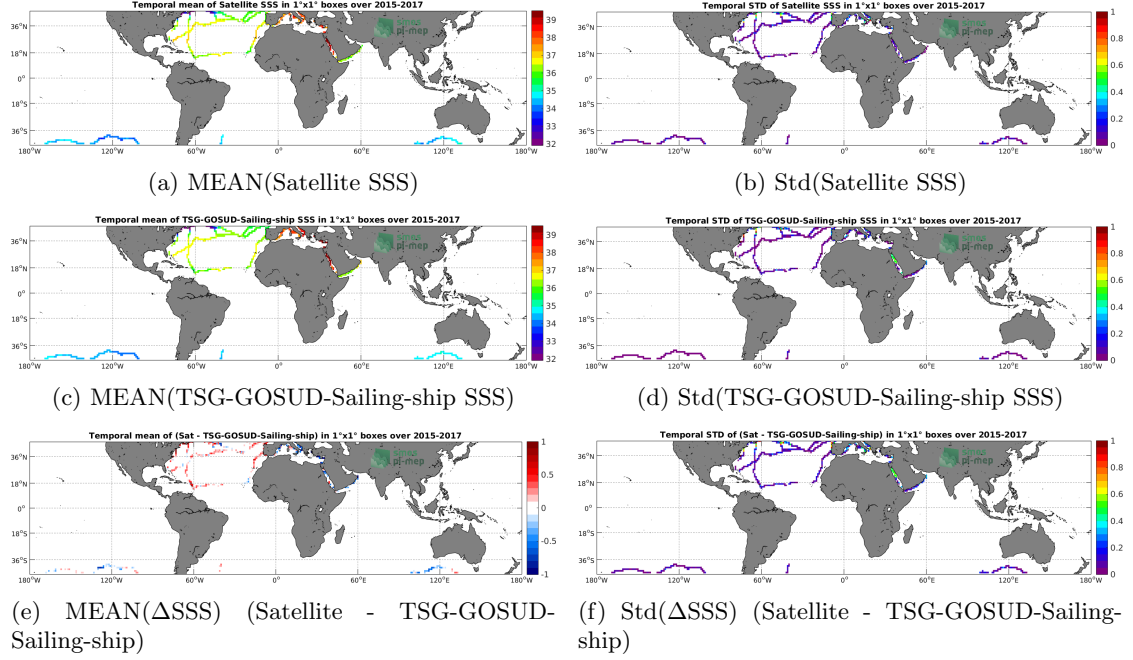
Figure 6: Temporal mean (left) and Std (right) of SSS from SMAP-L3-RSS-V4-8DAY-RUNNING (top), TSG-GOSUD-Sailing-ship (middle), and of \Delta SSS (Satellite - TSG-GOSUD-Sailing-ship). Only match-up pairs are used to generate these maps.
