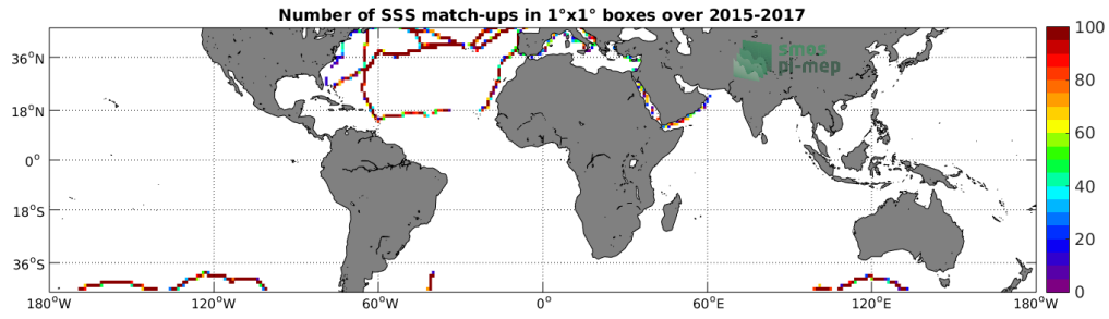
Figure 4: Number of SSS match-ups between TSG-GOSUD-Sailing-ship SSS and the SMAP-L3-RSS-V4-8DAY-RUNNING SSS product for the Mid-Low Latitudes 45N-45S Pi-MEP region over 1^\circ \times 1^\circ boxes and for the full satellite product period.
