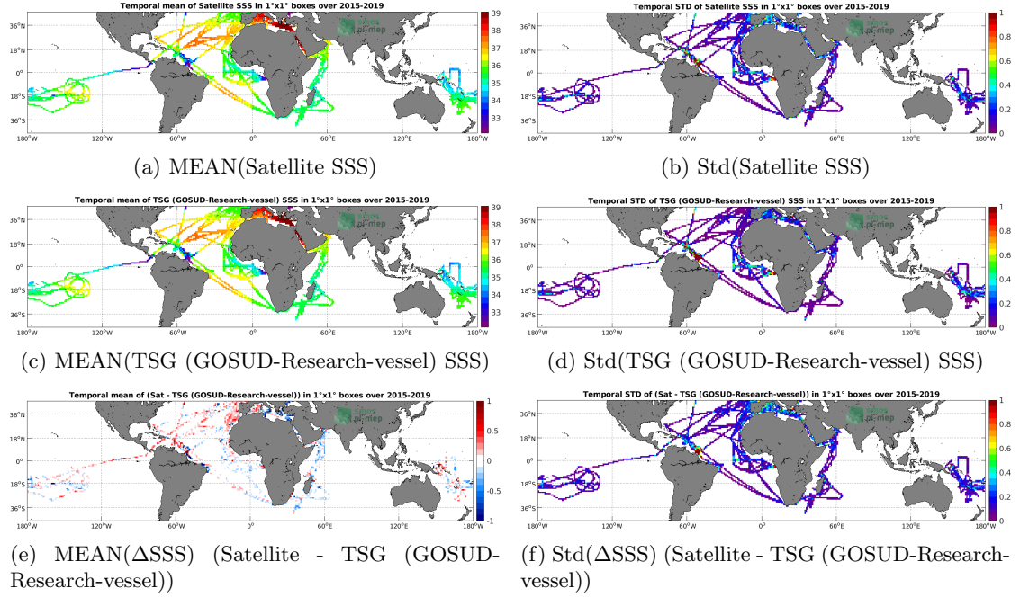
Figure 6: Temporal mean (left) and Std (right) of SSS from SMAP SSS L3 v4 - 8-Day running (RSS) (top), TSG (GOSUD-Research-vessel) (middle), and of \Delta SSS (Satellite - TSG (GOSUD-Research-vessel)). Only match-up pairs are used to generate these maps.
