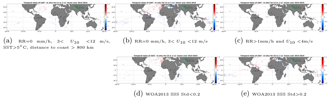
Figure 12: Temporal mean gridded over spatial boxes of size 1^\circ \times 1^\circ of \Delta SSS (SMAP SSS L3 v4 - 8-Day running (RSS) - TSG (GOSUD-Research-vessel)) for 5 different subdatasets corresponding to: RR=0 mm/h, 3 < U_{10} < 12 m/s, SST > 5^\circ C , distance to coast > 800 km (a), RR=0 mm/h, 3 < U_{10} < 12 m/s (b), RR > 1 mm/h and U_{10} < 4 m/s (c), WOA2013 SSS Std < 0.2 (d), WOA2013 SSS Std > 0.2 (e).
