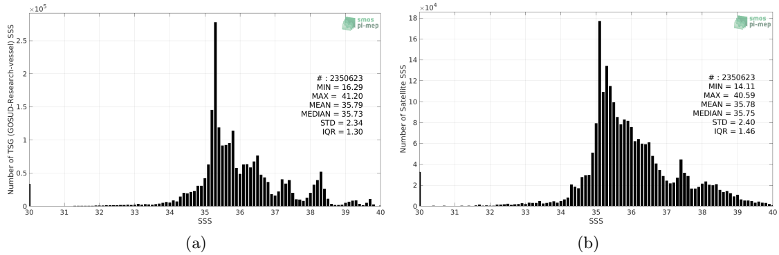
Figure 2: Histograms of SSS from TSG (GOSUD-Research-vessel) (a) and SMAP SSS L3 v4 - 8-Day running (RSS) (b) considering all match-up pairs per bins of 0.1 over the Mid-Low Latitudes 45N-45S Pi-MEP region and for the full satellite product period.
