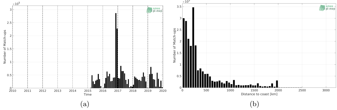
Figure 1: Number of match-ups between TSG (GOSUD-Research-vessel) and SMAP SSS L3 v4 - 8-Day running (RSS) SSS as a function of time (a) and as function of the distance to coast (b) over the Mid-Low Latitudes 45N-45S Pi-MEP region and for the full satellite product period.
