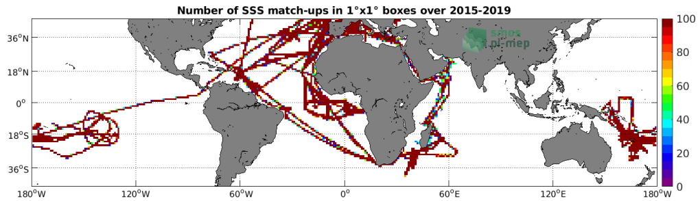
Figure 4: Number of SSS match-ups between TSG (GOSUD-Research-vessel) SSS and the SMAP SSS L3 v4 - 8-Day running (RSS) SSS product for the Mid-Low Latitudes 45N-45S Pi-MEP region over 1^\circ \times 1^\circ boxes and for the full satellite product period.
