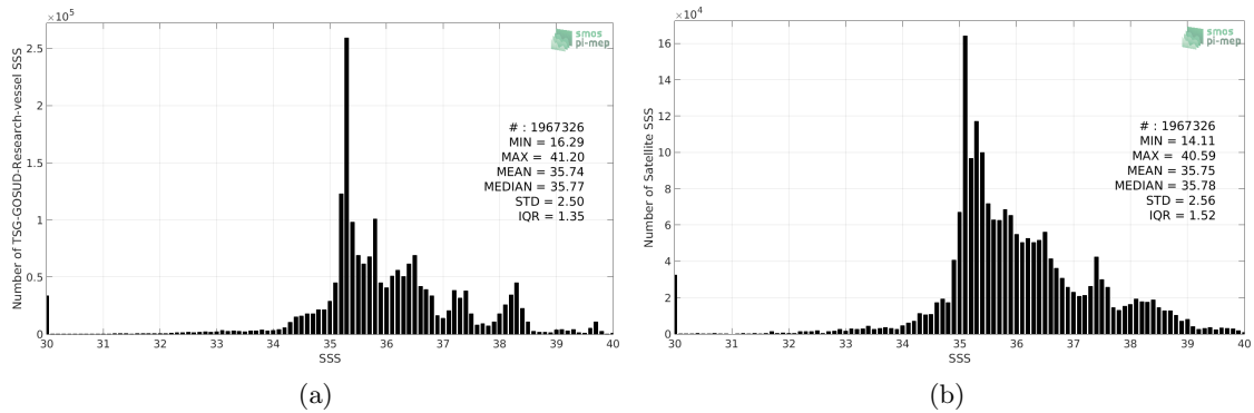
Figure 2: Histograms of SSS from TSG-GOSUD-Research-vessel (a) and SMAP-L3-RSS-V4-8DAY-RUNNING (b) considering all match-up pairs per bins of 0.1 over the Mid-Low Latitudes 45N-45S Pi-MEP region and for the full satellite product period.
