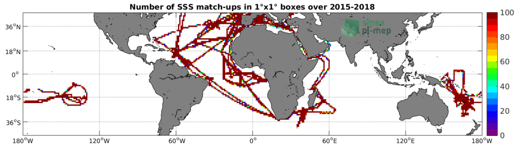
Figure 4: Number of SSS match-ups between TSG-GOSUD-Research-vessel SSS and the SMAP-L3-RSS-V4-8DAY-RUNNING SSS product for the Mid-Low Latitudes 45N-45S Pi-MEP region over 1^\circ \times 1^\circ boxes and for the full satellite product period.
