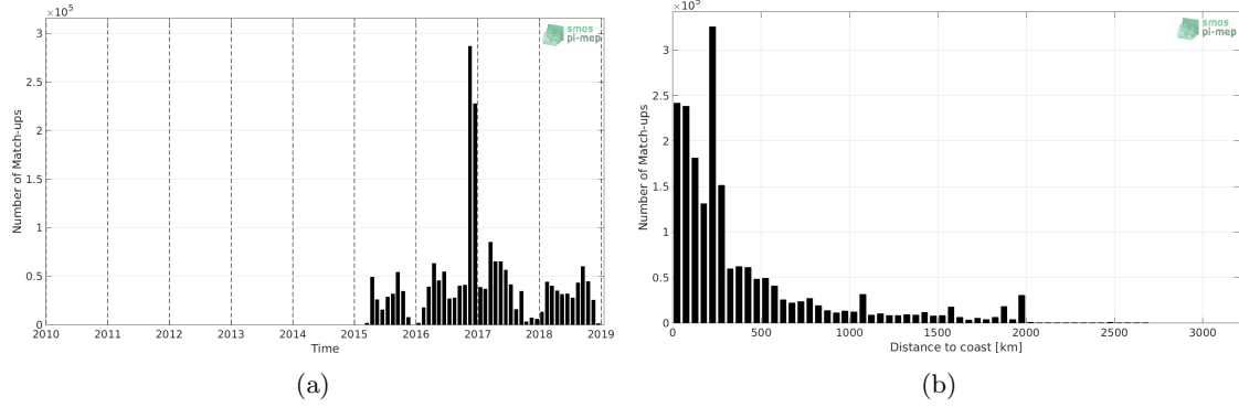
Figure 1: Number of match-ups between TSG-GOSUD-Research-vessel and SMAP-L3-RSS-V4-8DAY-RUNNING SSS as a function of time (a) and as function of the distance to coast (b) over the Mid-Low Latitudes 45N-45S Pi-MEP region and for the full satellite product period.
