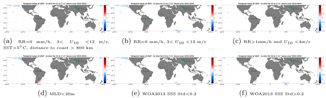
Figure 12: Temporal mean gridded over spatial boxes of size 1^\circ \times 1^\circ of \Delta SSS (SMAP SSS L3 v4 - 8-Day running (RSS) - Marine mammals) for 6 different subdatasets corresponding to:RR=0 mm/h, 3 < U_{10} < 12 m/s, SST >5^\circ C, distance to coast > 800 km (a), RR=0 mm/h, 3 < U_{10} < 12 m/s (b), RR >1 mm/h and U_{10} < 4 m/s (c),MLD <20 m (d),WOA2013 SSS Std <0.2 (e),WOA2013 SSS Std >0.2 (f).
