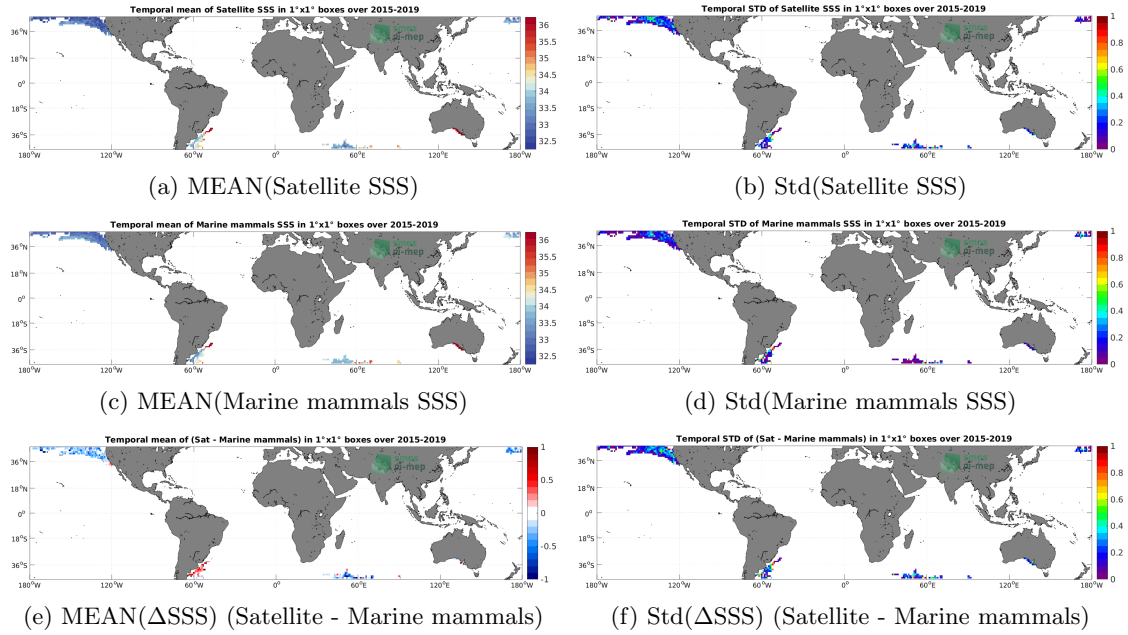
Figure 6: Temporal mean (left) and Std (right) of SSS from SMAP SSS L3 v4 - 8-Day running (RSS) (top), Marine mammals (middle), and of \Delta SSS (Satellite - Marine mammals). Only match-up pairs are used to generate these maps.
