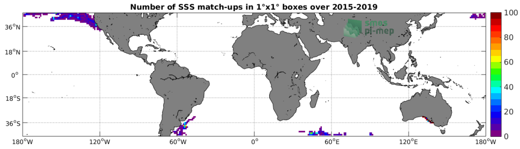
Figure 4: Number of SSS match-ups between Marine mammals SSS and the SMAP SSS L3 v4 - 8-Day running (RSS) SSS product for the Mid-Low Latitudes 45N-45S Pi-MEP region over 1^\circ \times 1^\circ boxes and for the full satellite product period.
