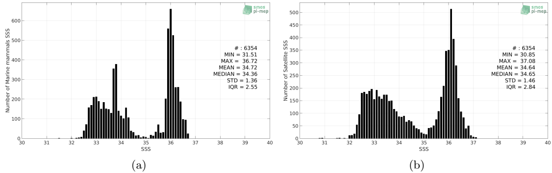
Figure 2: Histograms of SSS from Marine mammals (a) and SMAP SSS L3 v4 - 8-Day running (RSS) (b) considering all match-up pairs per bins of 0.1 over the Mid-Low Latitudes 45N-45S Pi-MEP region and for the full satellite product period.
