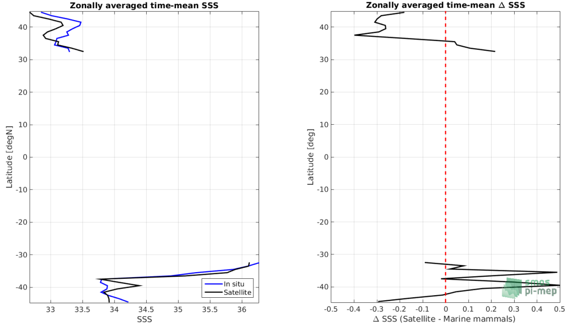
Figure 8: Left panel: Zonal mean SSS from SMAP SSS L3 v4 - 8-Day running (RSS) satellite product (black) and from Marine mammals (blue). Right panel: Zonal mean of \Delta SSS (Satellite - Marine mammals) for all the collected Pi-MEP match-up pairs estimated over the full satellite product period.
