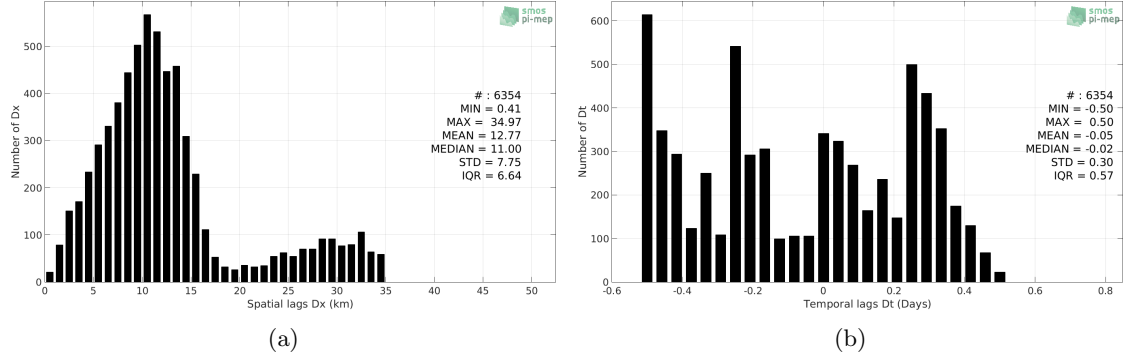
Figure 5: Histograms of the spatial (a) and temporal (b) lags between the location/time of the Marine mammals measurement and the date of the corresponding SMAP SSS L3 v4 - 8-Day running (RSS) SSS pixel.
