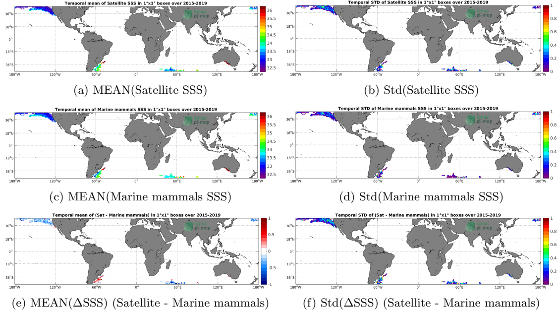
Figure 6: Temporal mean (left) and Std (right) of SSS from SMAP SSS L3 v4 - 8-Day running (RSS) (top), Marine mammals (middle), and of \Delta SSS (Satellite - Marine mammals). Only match-up pairs are used to generate these maps.
