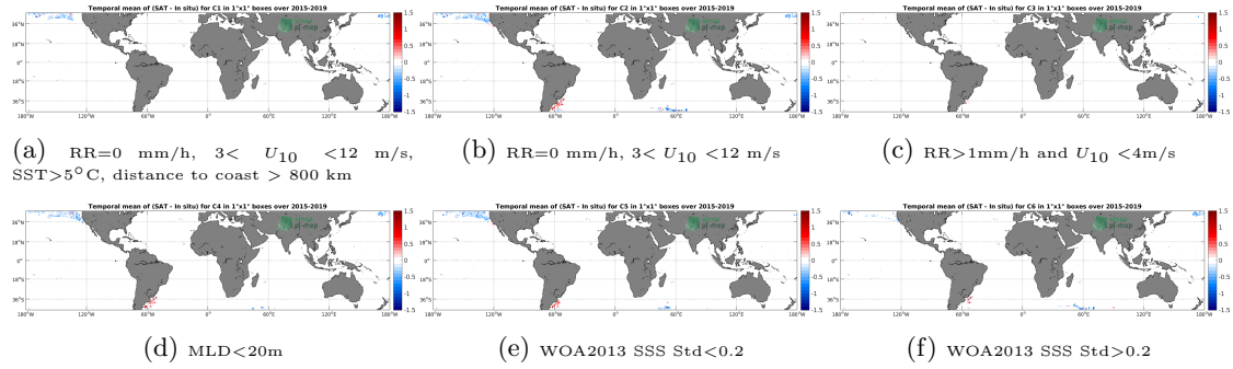
Figure 12: Temporal mean gridded over spatial boxes of size 1^\circ \times 1^\circ of \Delta SSS (SMAP SSS L3 v4 - 8-Day running (RSS) - Marine mammals) for 6 different subdatasets corresponding to: RR=0 mm/h, 3 < U_{10} < 12 m/s, SST > 5^\circ C , distance to coast > 800 km (a), RR=0 mm/h, 3 < U_{10} < 12 m/s (b), RR > 1 mm/h and U_{10} < 4 m/s (c), MLD < 20 m (d), WOA2013 SSS Std < 0.2 (e), WOA2013 SSS Std > 0.2 (f).
