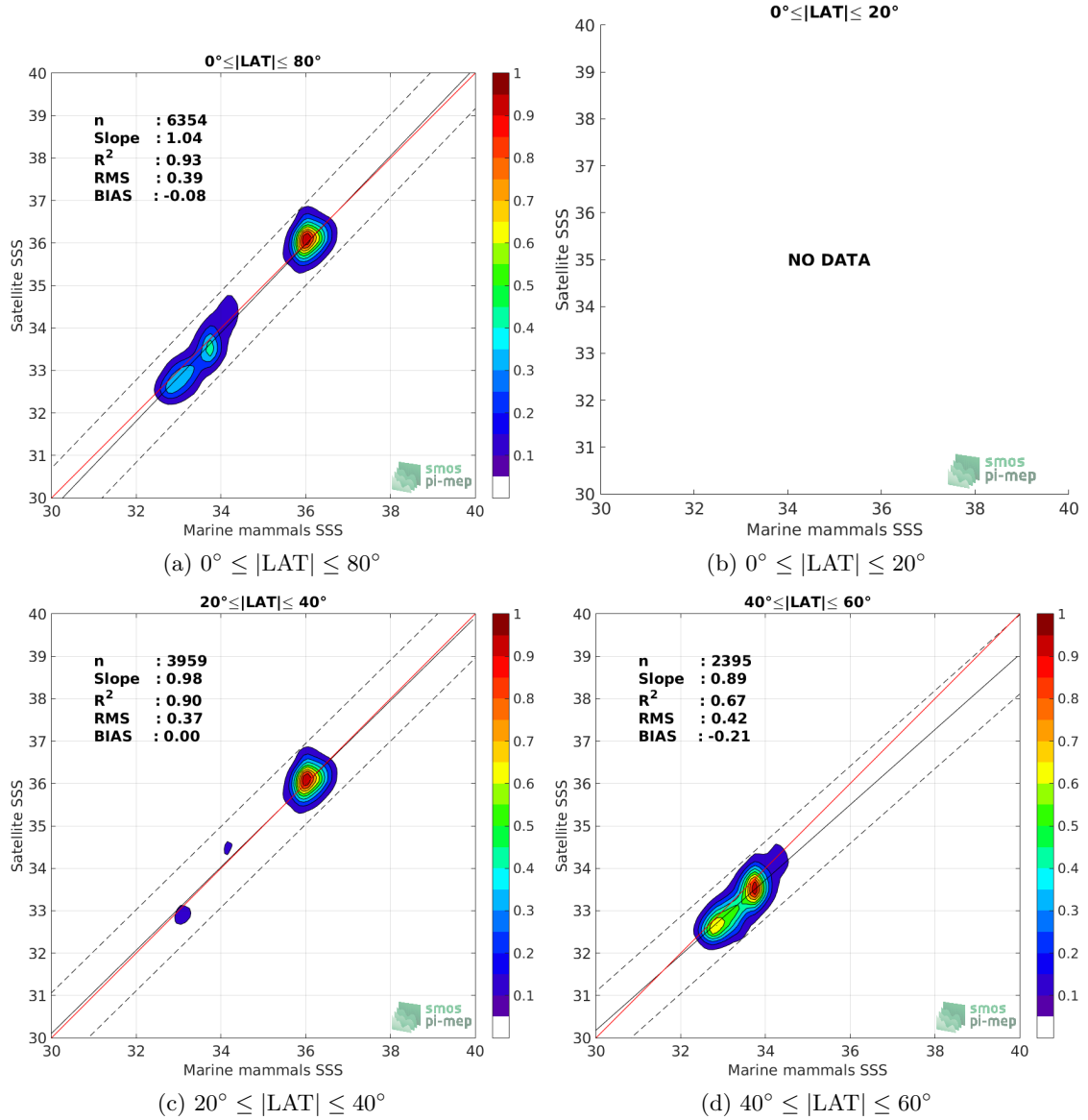
Figure 9: Contour maps of the concentration of SMAP SSS L3 v4 - 8-Day running (RSS) SSS (y-axis) versus Marine mammals SSS (x-axis) at match-up pairs for different latitude bands. For each plot, the red line shows x=y . The black thin and dashed lines indicate a linear fit through the data cloud and the \pm 95\% confidence levels, respectively. The number match-up pairs n , the slope and R^2 coefficient of the linear fit, the root mean square (RMS) and the mean bias between satellite and in situ data are indicated for each latitude band in each plots.
