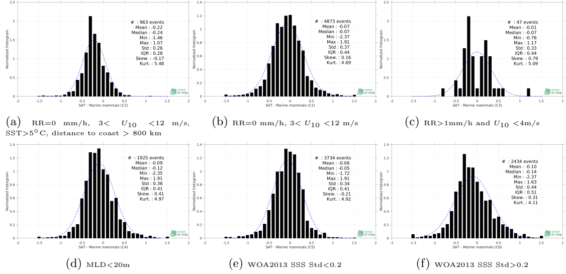
Figure 13: Normalized histogram of \Delta SSS (SMAP SSS L3 v4 - 8-Day running (RSS) - Marine mammals) for 6 different subdatasets corresponding to: RR=0 mm/h, 3 < U_{10} < 12 m/s, SST>5°C, distance to coast > 800 km (a), RR=0 mm/h, 3 < U_{10} < 12 m/s (b), RR>1mm/h and U_{10} < 4 m/s (c), MLD<20m (d), WOA2013 SSS Std<0.2 (e), WOA2013 SSS Std>0.2 (f).
