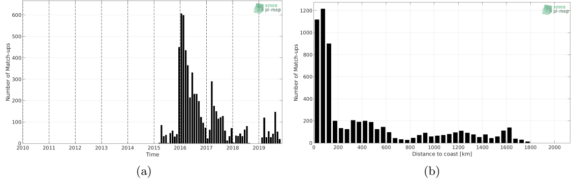
Figure 1: Number of match-ups between Marine mammals and SMAP SSS L3 v4 - 8-Day running (RSS) SSS as a function of time (a) and as function of the distance to coast (b) over the Mid-Low Latitudes 45N-45S Pi-MEP region and for the full satellite product period.
