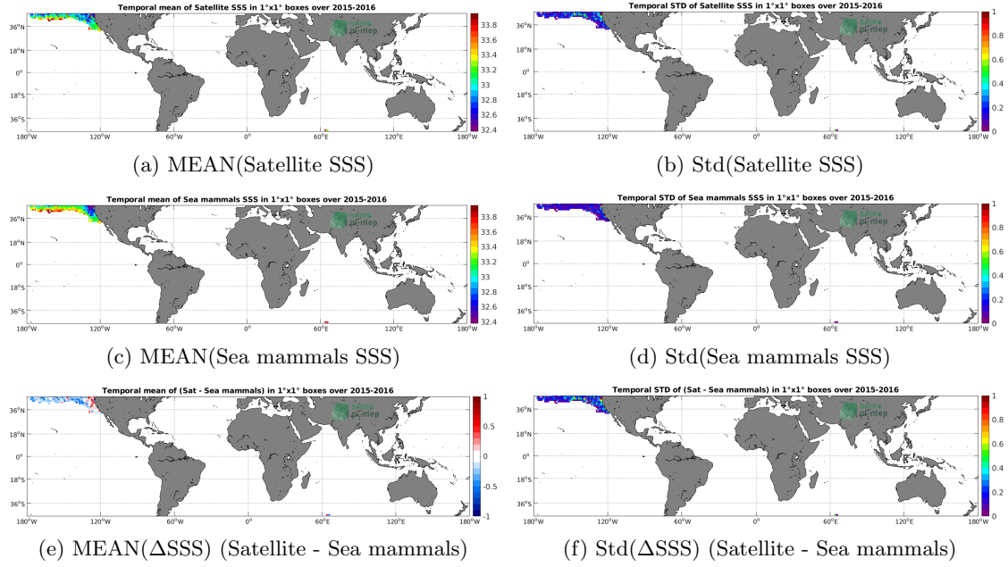
Figure 6: Temporal mean (left) and Std (right) of SSS from SMAP SSS L3 v4 - 8-Day running (RSS) (top), Sea mammals (middle), and of \Delta SSS (Satellite - Sea mammals). Only match-up pairs are used to generate these maps.
