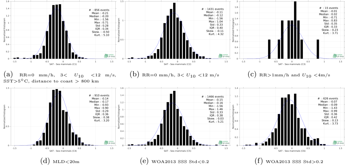
Figure 13: Normalized histogram of \Delta\text{SSS} (SMAP SSS L3 v4 - 8-Day running (RSS) - Sea mammals) for 6 different subdatasets corresponding to: RR=0 mm/h, 3 < U_{10} < 12 m/s, SST>5°C, distance to coast > 800 km (a), RR=0 mm/h, 3 < U_{10} < 12 m/s (b), RR>1mm/h and U_{10} < 4 m/s (c), MLD<20m (d), WOA2013 SSS Std<0.2 (e), WOA2013 SSS Std>0.2 (f).
