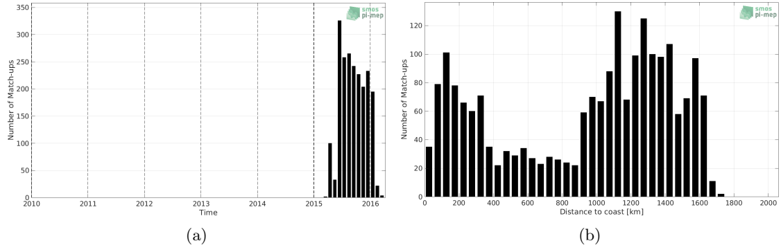
Figure 1: Number of match-ups between Sea mammals and SMAP SSS L3 v4 - 8-Day running (RSS) SSS as a function of time (a) and as function of the distance to coast (b) over the Mid-Low Latitudes 45N-45S Pi-MEP region and for the full satellite product period.
