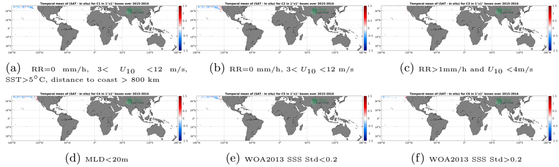
Figure 12: Temporal mean gridded over spatial boxes of size 1^\circ \times 1^\circ of \Delta SSS (SMAP SSS L3 v4 - 8-Day running (RSS) - Sea mammals) for 6 different subdatasets corresponding to: RR=0 mm/h, 3 < U_{10} < 12 m/s, SST > 5^\circ\text{C} , distance to coast > 800 km (a), RR=0 mm/h, 3 < U_{10} < 12 m/s (b), RR > 1 mm/h and U_{10} < 4 m/s (c), MLD < 20 m (d), WOA2013 SSS Std < 0.2 (e), WOA2013 SSS Std > 0.2 (f).
