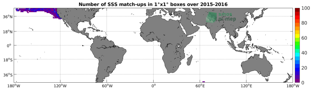
Figure 4: Number of SSS match-ups between Sea mammals SSS and the SMAP SSS L3 v4 - 8-Day running (RSS) SSS product for the Mid-Low Latitudes 45N-45S Pi-MEP region over 1^\circ \times 1^\circ boxes and for the full satellite product period.
