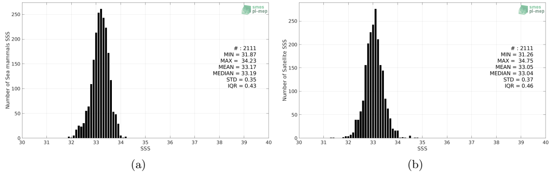
Figure 2: Histograms of SSS from Sea mammals (a) and SMAP SSS L3 v4 - 8-Day running (RSS) (b) considering all match-up pairs per bins of 0.1 over the Mid-Low Latitudes 45N-45S Pi-MEP region and for the full satellite product period.
