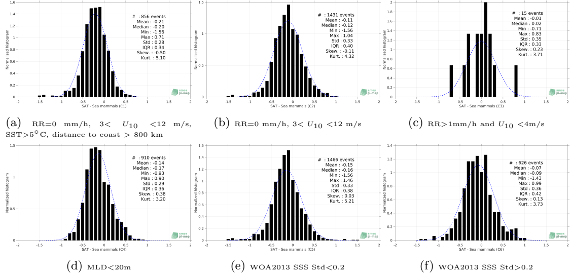
Figure 13: Normalized histogram of \Delta\text{SSS} (SMAP SSS L3 v4 - 8-Day running (RSS) - Sea mammals) for 6 different subdatasets corresponding to: RR=0 mm/h, 3 < U_{10} < 12 m/s, SST>5°C, distance to coast > 800 km (a), RR=0 mm/h, 3 < U_{10} < 12 m/s (b), RR>1mm/h and U_{10} < 4 m/s (c), MLD<20m (d), WOA2013 SSS Std<0.2 (e), WOA2013 SSS Std>0.2 (f).
