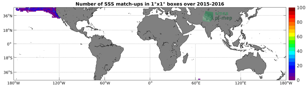
Figure 4: Number of SSS match-ups between Sea mammals SSS and the SMAP SSS L3 v4 - 8-Day running (RSS) SSS product for the Mid-Low Latitudes 45N-45S Pi-MEP region over 1°x1° boxes and for the full satellite product period.
