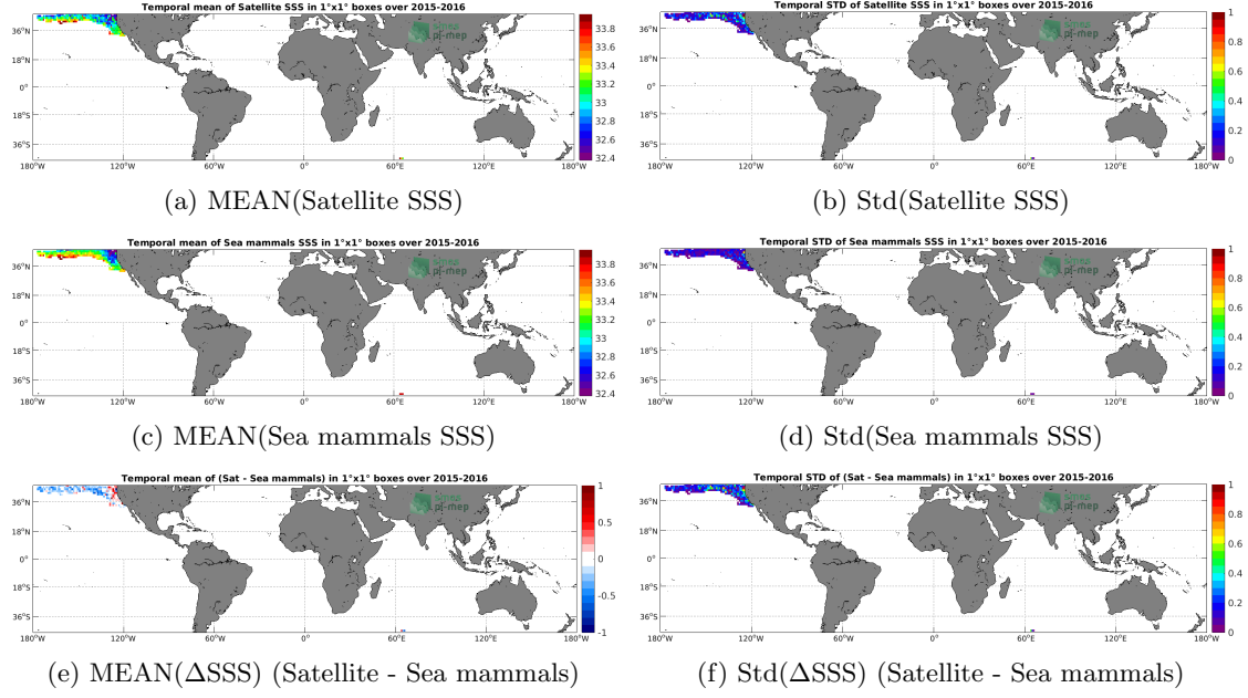
Figure 6: Temporal mean (left) and Std (right) of SSS from SMAP SSS L3 v4 - 8-Day running (RSS) (top), Sea mammals (middle), and of \Delta SSS (Satellite - Sea mammals). Only match-up pairs are used to generate these maps.
