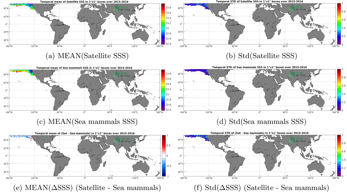
Figure 6: Temporal mean (left) and Std (right) of SSS from SMAP-L3-RSS-V4-8DAY-RUNNING (top), Sea mammals (middle), and of \Delta SSS (Satellite - Sea mammals). Only match-up pairs are used to generate these maps.
