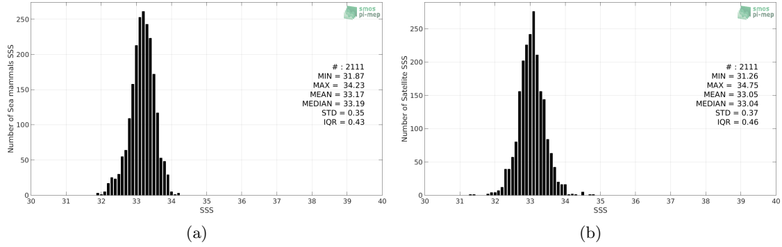
Figure 2: Histograms of SSS from Sea mammals (a) and SMAP-L3-RSS-V4-8DAY-RUNNING (b) considering all match-up pairs per bins of 0.1 over the Mid-Low Latitudes 45N-45S Pi-MEP region and for the full satellite product period.
