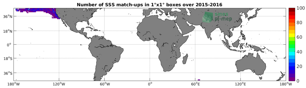
Figure 4: Number of SSS match-ups between Sea mammals SSS and the SMAP-L3-RSS-V4-8DAY-RUNNING SSS product for the Mid-Low Latitudes 45N-45S Pi-MEP region over 1^\circ \times 1^\circ boxes and for the full satellite product period.
