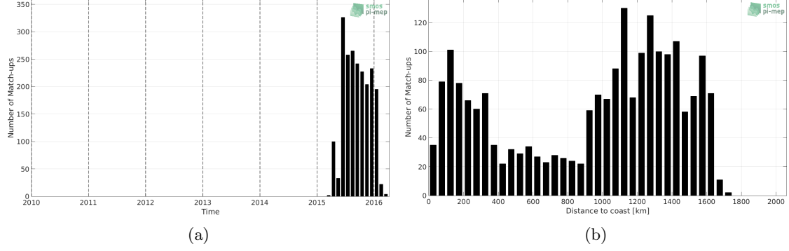
Figure 1: Number of match-ups between Sea mammals and SMAP-L3-RSS-V4-8DAY-RUNNING SSS as a function of time (a) and as function of the distance to coast (b) over the Mid-Low Latitudes 45N-45S Pi-MEP region and for the full satellite product period.
