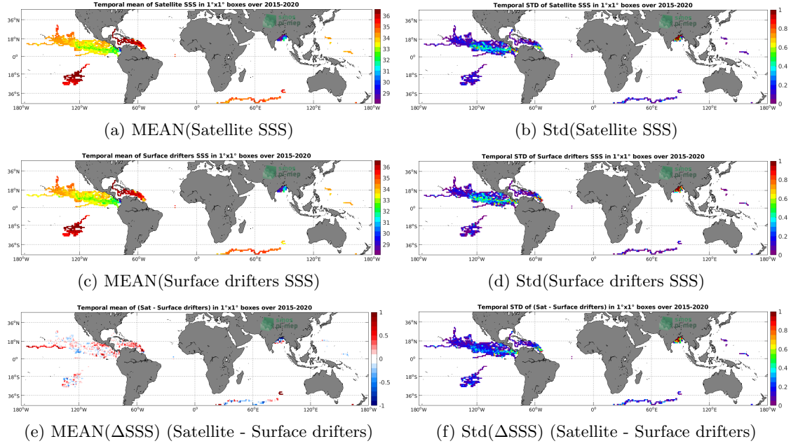
Figure 5: Temporal mean (left) and Std (right) of SSS from SMAP SSS L3 v4 - 8-Day running (RSS) (top), Surface drifters (middle), and of \Delta SSS (Satellite - Surface drifters). Only match-up pairs are used to generate these maps.
