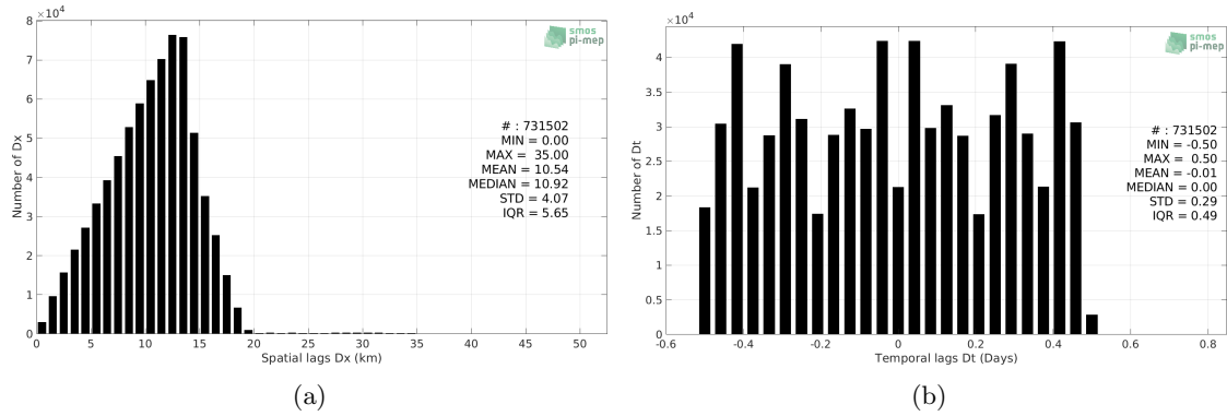
Figure 4: Histograms of the spatial (a) and temporal (b) lags between the location/time of the Surface drifters measurement and the date of the corresponding SMAP SSS L3 v4 - 8-Day running (RSS) SSS pixel.
