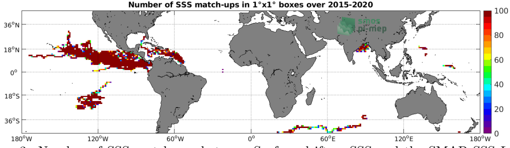
Figure 3: Number of SSS match-ups between Surface drifters SSS and the SMAP SSS L3 v4 - 8-Day running (RSS) SSS product for the Mid-Low Latitudes 45N-45S Pi-MEP region over 1^\circ \times 1^\circ boxes and for the full satellite product period.
