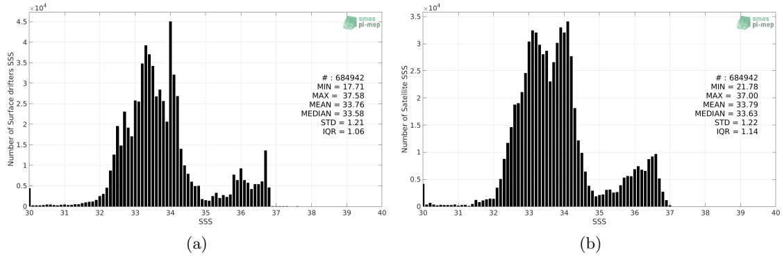
Figure 2: Histograms of SSS from Surface drifters (a) and SMAP SSS L3 v4 - 8-Day running (RSS) (b) considering all match-up pairs per bins of 0.1 over the Mid-Low Latitudes 45N-45S Pi-MEP region and for the full satellite product period.
