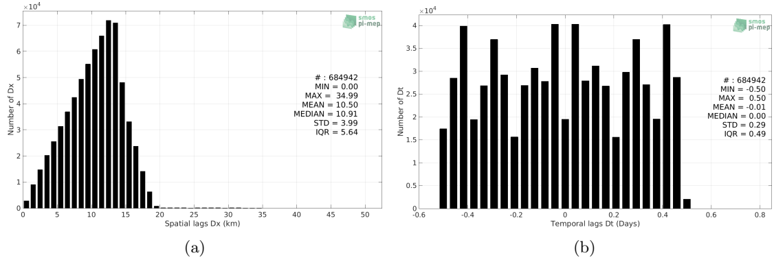
Figure 4: Histograms of the spatial (a) and temporal (b) lags between the time of the Surface drifters measurements and the date of the corresponding SMAP SSS L3 v4 - 8-Day running (RSS) SSS product.
