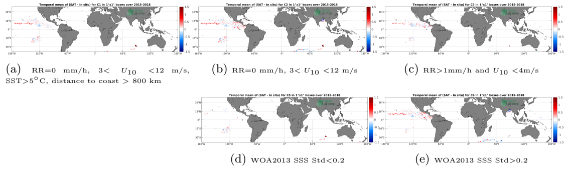
Figure 11: Temporal mean gridded over spatial boxes of size 1^\circ \times 1^\circ of \Delta SSS (SMAP SSS L3 v4 - 8-Day running (RSS) - Surface drifters) for 5 different subdatasets corresponding to: RR=0 mm/h, 3 < U_{10} < 12 m/s, SST > 5^\circ C , distance to coast > 800 km (a), RR=0 mm/h, 3 < U_{10} < 12 m/s (b), RR > 1 mm/h and U_{10} < 4 m/s (c), WOA2013 SSS Std < 0.2 (d), WOA2013 SSS Std > 0.2 (e).
