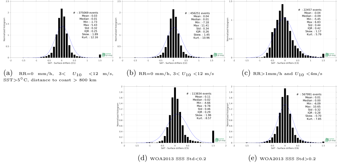
Figure 12: Normalized histogram of \Delta SSS (SMAP SSS L3 v4 - 8-Day running (RSS) - Surface drifters) for 5 different subdatasets corresponding to: RR=0 mm/h, 3 < U_{10} < 12 m/s, SST>5°C, distance to coast > 800 km (a), RR=0 mm/h, 3 < U_{10} < 12 m/s (b), RR>1mm/h and U_{10} < 4 m/s (c), WOA2013 SSS Std<0.2 (d), WOA2013 SSS Std>0.2 (e).
