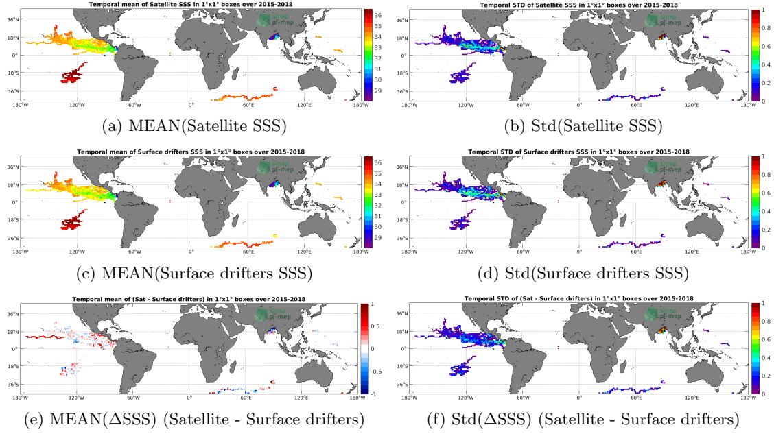
Figure 5: Temporal mean (left) and Std (right) of SSS from SMAP SSS L3 v4 - 8-Day running (RSS) (top), Surface drifters (middle), and of \Delta SSS (Satellite - Surface drifters). Only match-up pairs are used to generate these maps.
