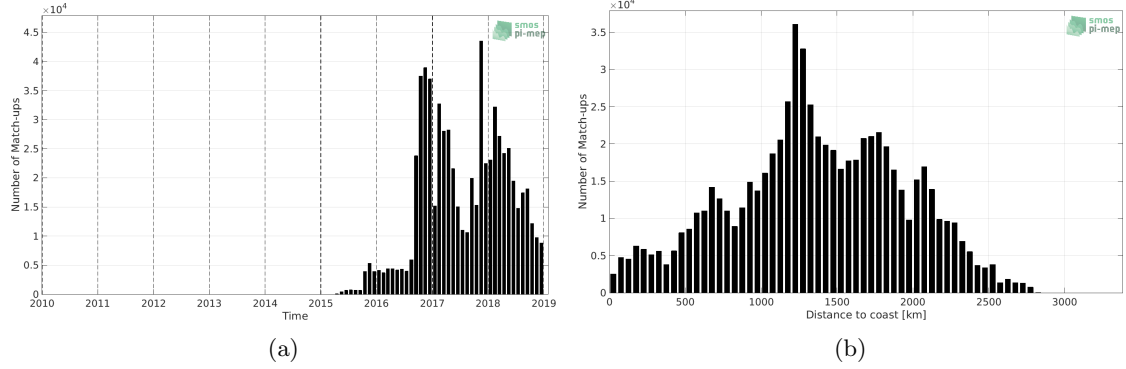
Figure 1: Number of match-ups between Surface drifters and SMAP SSS L3 v4 - 8-Day running (RSS) SSS as a function of time (a) and as function of the distance to coast (b) over the Mid-Low Latitudes 45N-45S Pi-MEP region and for the full satellite product period.
