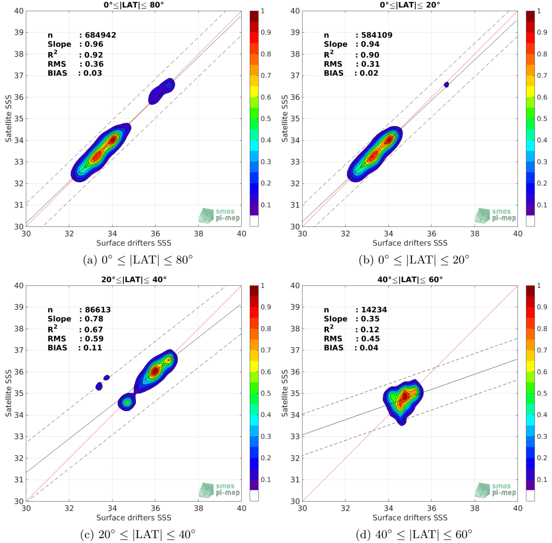
Figure 8: Contour maps of the concentration of SMAP SSS L3 v4 - 8-Day running (RSS) SSS (y-axis) versus Surface drifters SSS (x-axis) at match-up pairs for different latitude bands. For each plot, the red line shows x=y . The black thin and dashed lines indicate a linear fit through the data cloud and the \pm 95\% confidence levels, respectively. The number match-up pairs n , the slope and R^2 coefficient of the linear fit, the root mean square (RMS) and the mean bias between satellite and in situ data are indicated for each latitude band in each plots.
