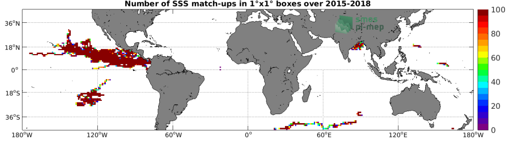
Figure 3: Number of SSS match-ups between Surface drifters SSS and the SMAP SSS L3 v4 - 8-Day running (RSS) SSS product for the Mid-Low Latitudes 45N-45S Pi-MEP region over 1°x1° boxes and for the full satellite product period.
