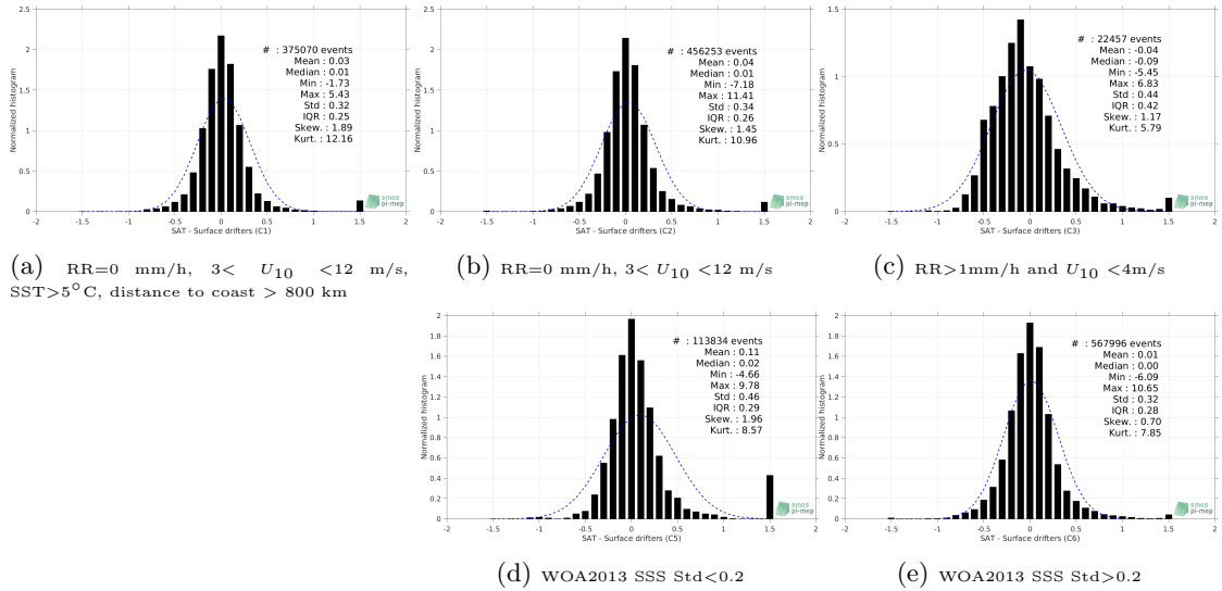
Figure 12: Normalized histogram of \Delta SSS (SMAP-L3-RSS-V4-8DAY-RUNNING - Surface drifters) for 5 different subdatasets corresponding to: RR=0 mm/h, 3 < U_{10} < 12 m/s, SST >5^\circ\text{C} , distance to coast > 800 km (a), RR=0 mm/h, 3 < U_{10} < 12 m/s (b), RR >1 mm/h and U_{10} < 4 m/s (c), WOA2013 SSS Std <0.2 (d), WOA2013 SSS Std >0.2 (e).
