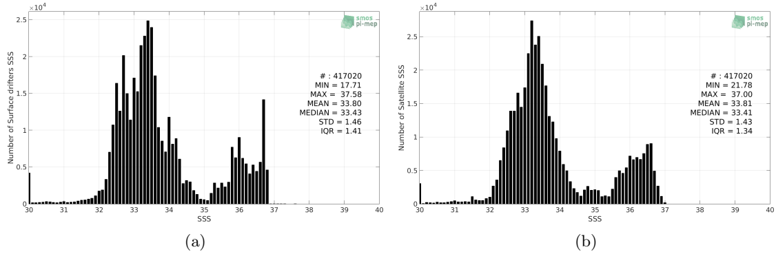
Figure 2: Histograms of SSS from Surface drifters (a) and SMAP-L3-RSS-V4-8DAY-RUNNING (b) considering all match-up pairs per bins of 0.1 over the Mid-Low Latitudes 45N-45S Pi-MEP region and for the full satellite product period.
