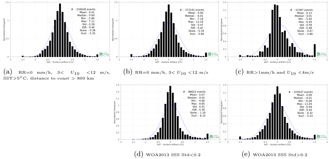
Figure 12: Normalized histogram of \Delta SSS (SMAP-L3-RSS-V4-8DAY-RUNNING - Surface drifters) for 5 different subdatasets corresponding to: RR=0 mm/h, 3 < U_{10} < 12 m/s, SST > 5^\circ C , distance to coast > 800 km (a), RR=0 mm/h, 3 < U_{10} < 12 m/s (b), RR > 1 mm/h and U_{10} < 4 m/s (c), WOA2013 SSS Std < 0.2 (d), WOA2013 SSS Std > 0.2 (e).
