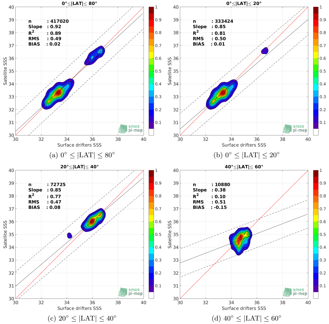
Figure 8: Contour maps of the concentration of SMAP-L3-RSS-V4-8DAY-RUNNING SSS (y-axis) versus Surface drifters SSS (x-axis) at match-up pairs for different latitude bands. For each plot, the red line shows x=y . The black thin and dashed lines indicate a linear fit through the data cloud and the \pm 95\% confidence levels, respectively. The number match-up pairs n , the slope and R^2 coefficient of the linear fit, the root mean square (RMS) and the mean bias between satellite and in situ data are indicated for each latitude band in each plots.
