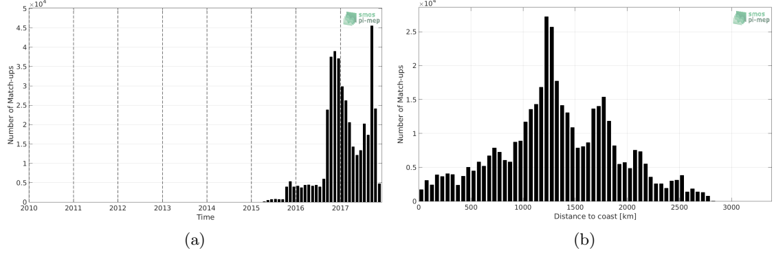
Figure 1: Number of match-ups between Surface drifters and SMAP-L3-RSS-V4-8DAY-RUNNING SSS as a function of time (a) and as function of the distance to coast (b) over the Mid-Low Latitudes 45N-45S Pi-MEP region and for the full satellite product period.
