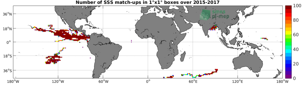
Figure 3: Number of SSS match-ups between Surface drifters SSS and the SMAP-L3-RSS-V4-8DAY-RUNNING SSS product for the Mid-Low Latitudes 45N-45S Pi-MEP region over 1^\circ \times 1^\circ boxes and for the full satellite product period.
