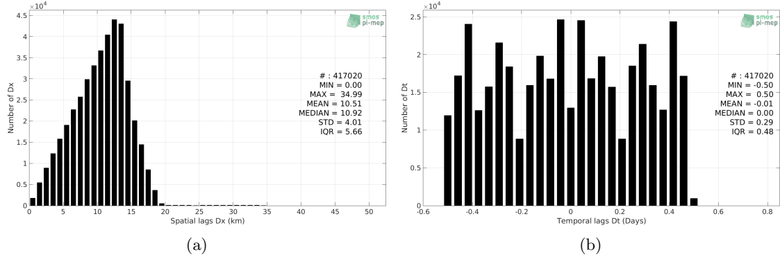
Figure 4: Histograms of the spatial (a) and temporal (b) lags between the time of the Surface drifters measurements and the date of the corresponding SMAP-L3-RSS-V4-8DAY-RUNNING SSS product.
