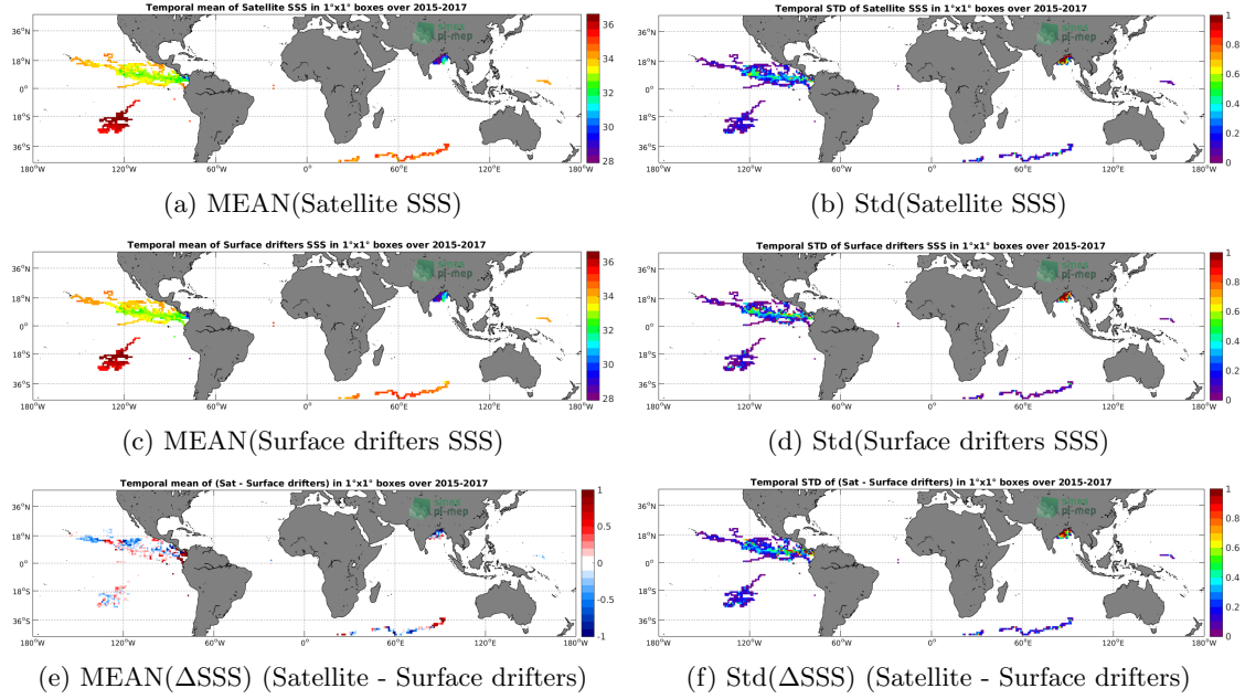
Figure 5: Temporal mean (left) and Std (right) of SSS from SMAP-L3-RSS-V4-8DAY-RUNNING (top), Surface drifters (middle), and of \Delta SSS (Satellite - Surface drifters). Only match-up pairs are used to generate these maps.
