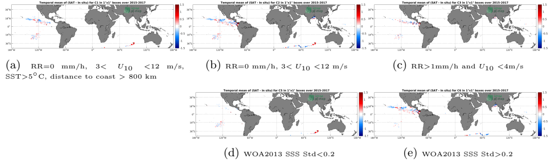
Figure 11: Temporal mean gridded over spatial boxes of size 1^\circ \times 1^\circ of \Delta SSS (SMAP-L3-RSS-V4-8DAY-RUNNING - Surface drifters) for 5 different subdatasets corresponding to: RR=0 mm/h, 3 < U_{10} < 12 m/s, SST > 5^\circ C , distance to coast > 800 km (a), RR=0 mm/h, 3 < U_{10} < 12 m/s (b), RR > 1 mm/h and U_{10} < 4 m/s (c), WOA2013 SSS Std < 0.2 (d), WOA2013 SSS Std > 0.2 (e).
