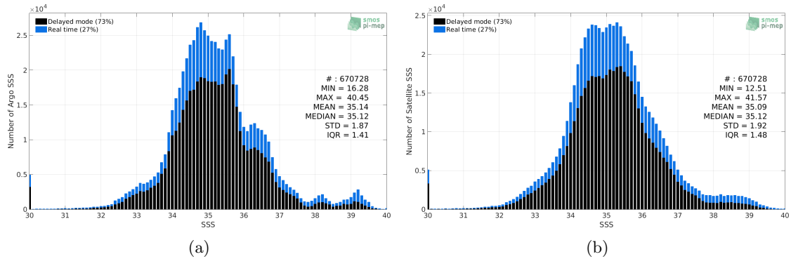
Figure 2: Histograms of SSS from Argo (a) and SMAP SSS L3 v4 - 8-Day running (RSS) (b) considering all match-up pairs per bins of 0.1 over the Mid-Low Latitudes 45N-45S Pi-MEP region and for the full satellite product period.
