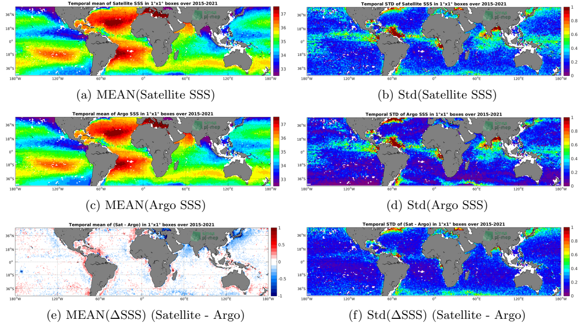
Figure 6: Temporal mean (left) and Std (right) of SSS from SMAP SSS L3 v4 - 8-Day running (RSS) (top), Argo (middle), and of \Delta SSS (Satellite - Argo). Only match-up pairs are used to generate these maps.
