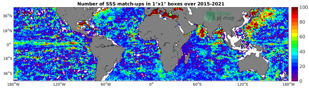
Figure 4: Number of SSS match-ups between Argo SSS and the SMAP SSS L3 v4 - 8-Day running (RSS) SSS product for the Mid-Low Latitudes 45N-45S Pi-MEP region over 1^\circ \times 1^\circ boxes and for the full satellite product period.
