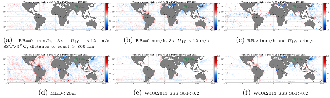
Figure 12: Temporal mean gridded over spatial boxes of size 1^\circ \times 1^\circ of \Delta SSS (SMAP SSS L3 v4 - 8-Day running (RSS) - Argo) for 6 different subdatasets corresponding to: RR=0 mm/h, 3 < U_{10} < 12 m/s, SST > 5^\circ\text{C} , distance to coast > 800 km (a), RR=0 mm/h, 3 < U_{10} < 12 m/s (b), RR > 1 mm/h and U_{10} < 4 m/s (c), MLD < 20 m (d), WOA2013 SSS Std < 0.2 (e), WOA2013 SSS Std > 0.2 (f).
