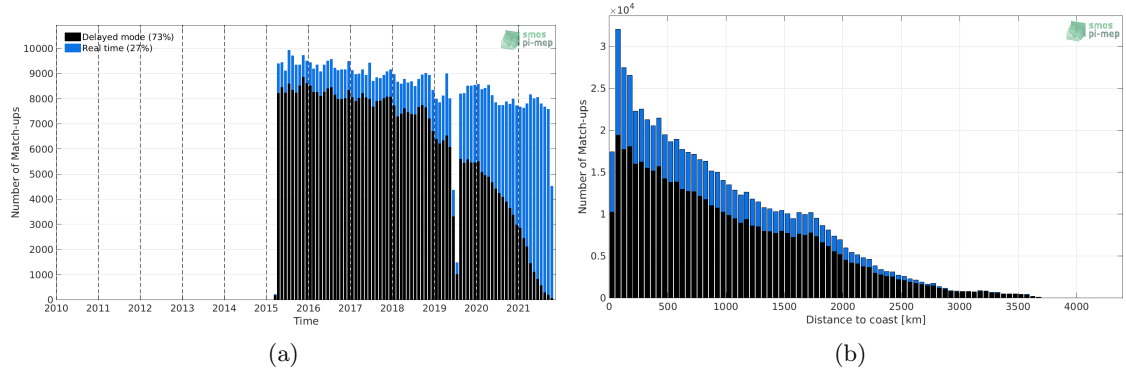
Figure 1: Number of match-ups between Argo and SMAP SSS L3 v4 - 8-Day running (RSS) SSS as a function of time (a) and as function of the distance to coast (b) over the Mid-Low Latitudes 45N-45S Pi-MEP region and for the full satellite product period.
