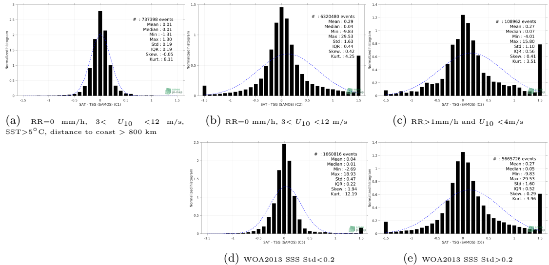
Figure 13: Normalized histogram of \Delta SSS (SMAP SSS L3 v4 - Monthly (RSS) - TSG (SAMOS)) for 5 different subdatasets corresponding to: RR=0 mm/h, 3 < U_{10} < 12 m/s, SST >5^\circ\text{C} , distance to coast > 800 km (a), RR=0 mm/h, 3 < U_{10} < 12 m/s (b), RR >1 mm/h and U_{10} < 4 m/s (c), WOA2013 SSS Std <0.2 (d), WOA2013 SSS Std >0.2 (e).
