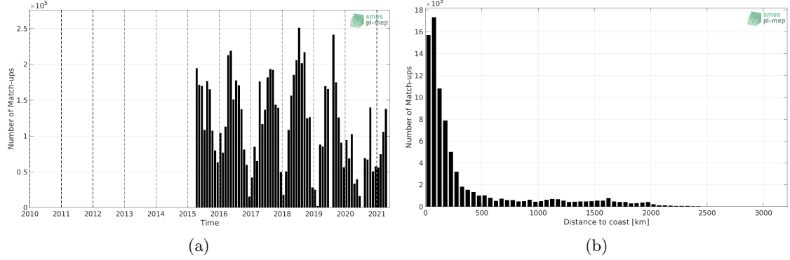
Figure 1: Number of match-ups between TSG (SAMOS) and SMAP SSS L3 v4 - Monthly (RSS) SSS as a function of time (a) and as function of the distance to coast (b) over the Mid-Low Latitudes 45N-45S Pi-MEP region and for the full satellite product period.
