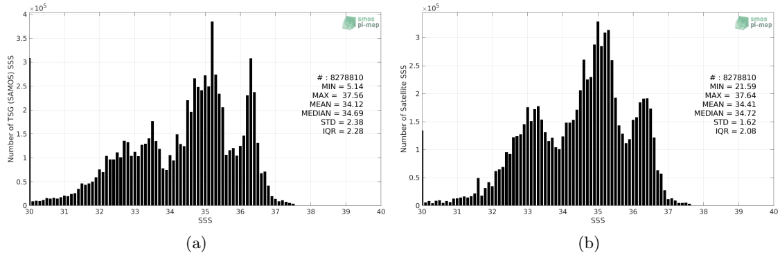
Figure 2: Histograms of SSS from TSG (SAMOS) (a) and SMAP SSS L3 v4 - Monthly (RSS) (b) considering all match-up pairs per bins of 0.1 over the Mid-Low Latitudes 45N-45S Pi-MEP region and for the full satellite product period.
