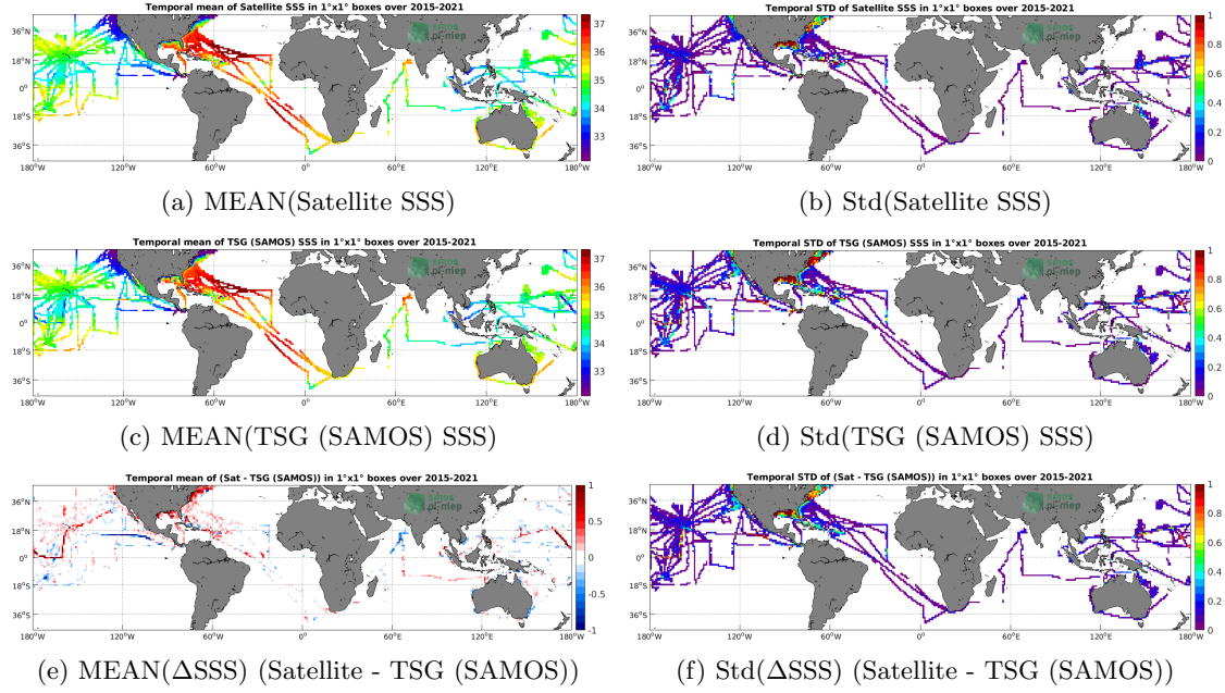
Figure 6: Temporal mean (left) and Std (right) of SSS from SMAP SSS L3 v4 - Monthly (RSS) (top), TSG (SAMOS) (middle), and of \Delta SSS (Satellite - TSG (SAMOS)). Only match-up pairs are used to generate these maps.
