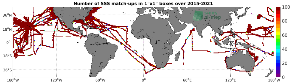
Figure 4: Number of SSS match-ups between TSG (SAMOS) SSS and the SMAP SSS L3 v4 - Monthly (RSS) SSS product for the Mid-Low Latitudes 45N-45S Pi-MEP region over 1^\circ \times 1^\circ boxes and for the full satellite product period.
