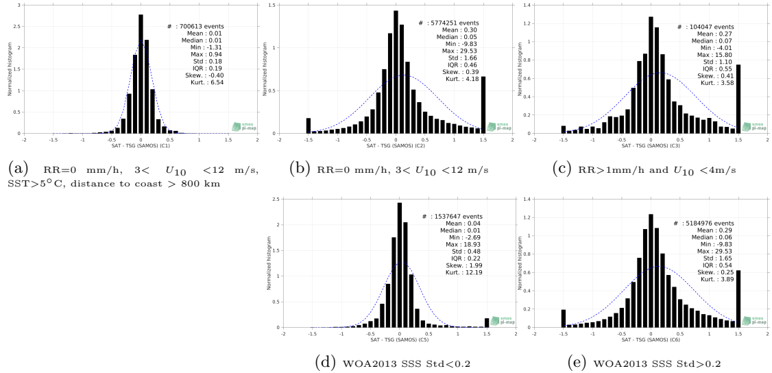
Figure 13: Normalized histogram of \Delta SSS (SMAP SSS L3 v4 - Monthly (RSS) - TSG (SAMOS)) for 5 different subdatasets corresponding to: RR=0 mm/h, 3 < U_{10} < 12 m/s, SST > 5^\circ C , distance to coast > 800 km (a), RR=0 mm/h, 3 < U_{10} < 12 m/s (b), RR > 1 mm/h and U_{10} < 4 m/s (c), WOA2013 SSS Std < 0.2 (d), WOA2013 SSS Std > 0.2 (e).
