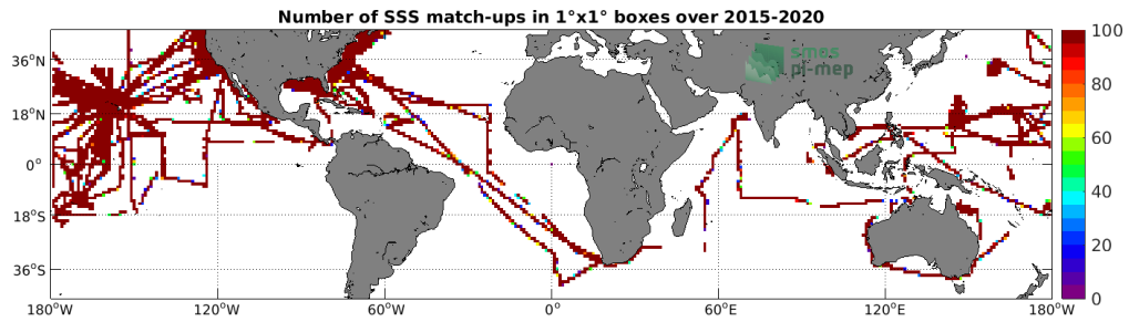
Figure 4: Number of SSS match-ups between TSG (SAMOS) SSS and the SMAP SSS L3 v4 - Monthly (RSS) SSS product for the Mid-Low Latitudes 45N-45S Pi-MEP region over 1°x1° boxes and for the full satellite product period.
