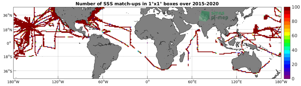
Figure 4: Number of SSS match-ups between TSG-SAMOS SSS and the SMAP-L3-RSS-V4-MONTHLY SSS product for the Mid-Low Latitudes 45N-45S Pi-MEP region over 1^\circ \times 1^\circ boxes and for the full satellite product period.
