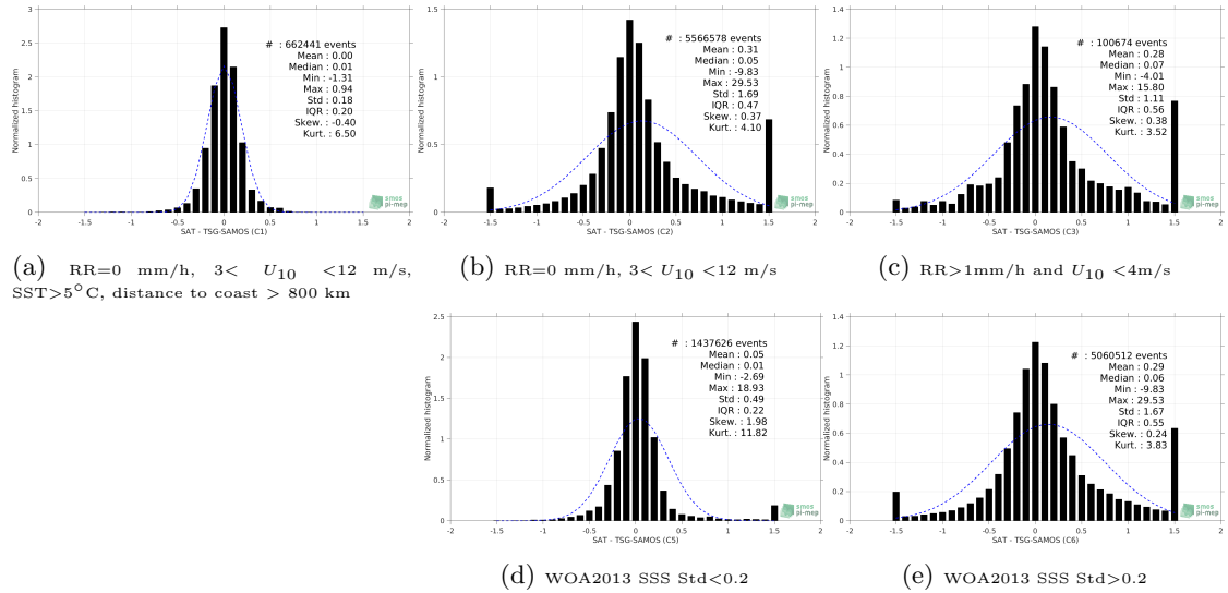
Figure 13: Normalized histogram of \Delta SSS (SMAP-L3-RSS-V4-MONTHLY - TSG-SAMOS) for 5 different subdatasets corresponding to: RR=0 mm/h, 3 < U_{10} < 12 m/s, SST >5^\circ\text{C} , distance to coast > 800 km (a), RR=0 mm/h, 3 < U_{10} < 12 m/s (b), RR >1 mm/h and U_{10} < 4 m/s (c), WOA2013 SSS Std <0.2 (d), WOA2013 SSS Std >0.2 (e).
