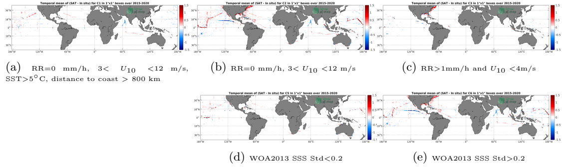
Figure 12: Temporal mean gridded over spatial boxes of size 1^\circ \times 1^\circ of \Delta SSS (SMAP-L3-RSS-V4-MONTHLY - TSG-SAMOS) for 5 different subdatasets corresponding to:RR=0 mm/h, 3 < U_{10} < 12 m/s, SST >5^\circ\text{C} , distance to coast > 800 km (a), RR=0 mm/h, 3 < U_{10} < 12 m/s (b), RR >1 mm/h and U_{10} < 4 m/s (c), WOA2013 SSS Std <0.2 (d), WOA2013 SSS Std >0.2 (e).
