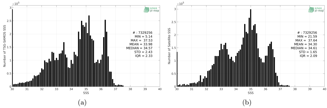
Figure 2: Histograms of SSS from TSG-SAMOS (a) and SMAP-L3-RSS-V4-MONTHLY (b) considering all match-up pairs per bins of 0.1 over the Mid-Low Latitudes 45N-45S Pi-MEP region and for the full satellite product period.
