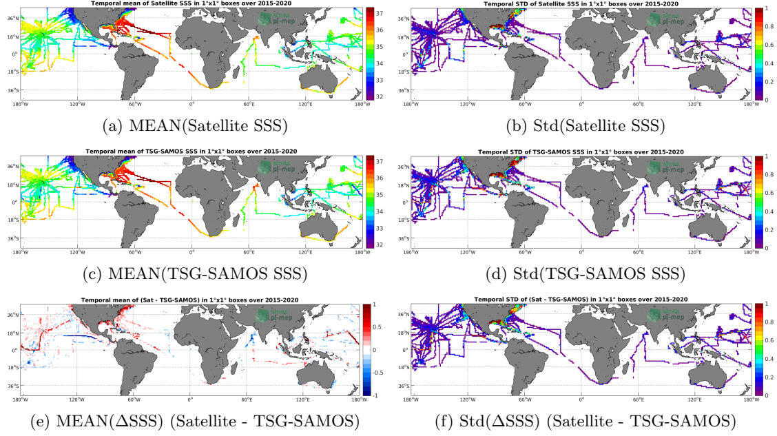
Figure 6: Temporal mean (left) and Std (right) of SSS from SMAP-L3-RSS-V4-MONTHLY (top), TSG-SAMOS (middle), and of \Delta SSS (Satellite - TSG-SAMOS). Only match-up pairs are used to generate these maps.
