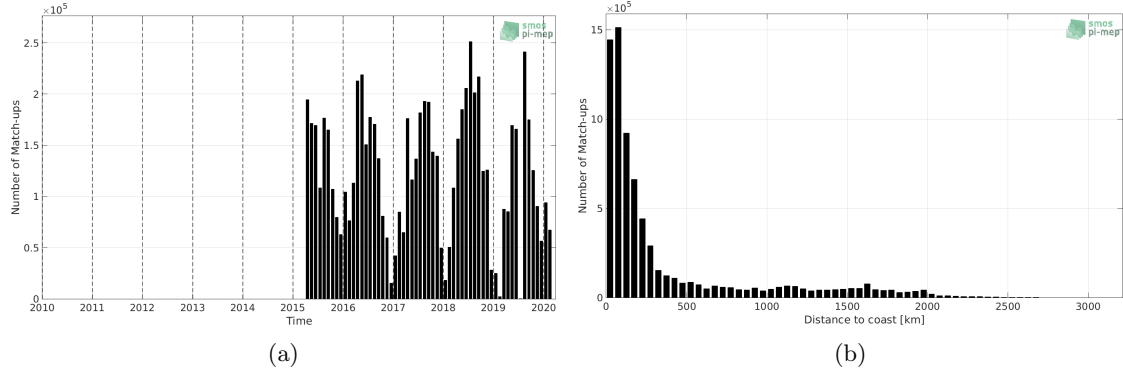
Figure 1: Number of match-ups between TSG-SAMOS and SMAP-L3-RSS-V4-MONTHLY SSS as a function of time (a) and as function of the distance to coast (b) over the Mid-Low Latitudes 45N-45S Pi-MEP region and for the full satellite product period.
