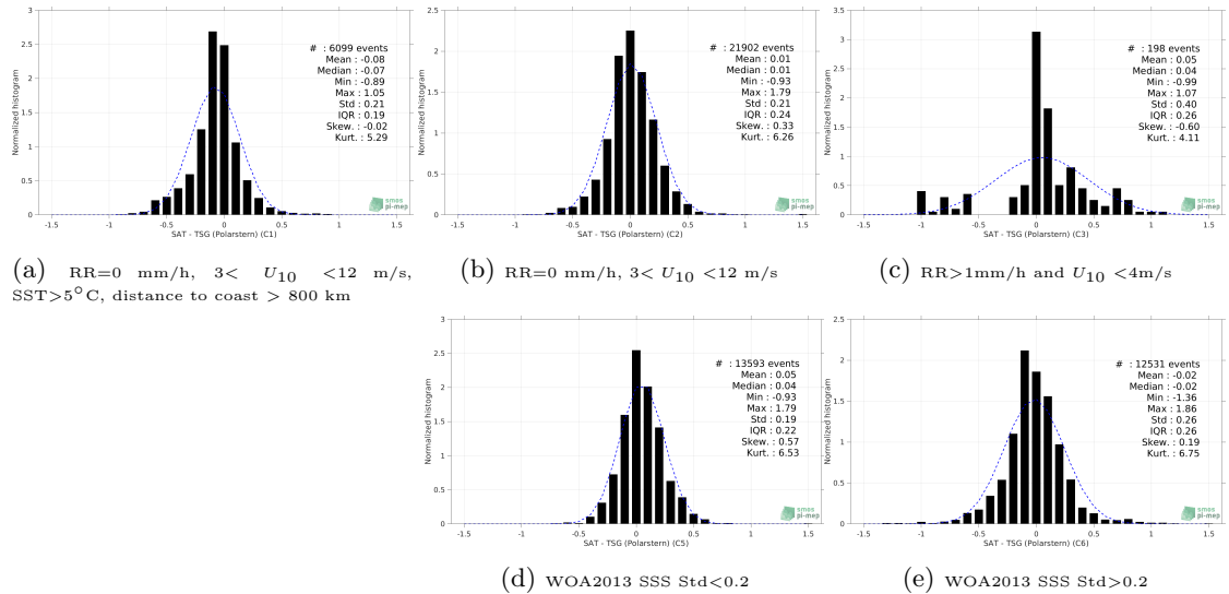
Figure 13: Normalized histogram of \Delta SSS (SMAP SSS L3 v4 - Monthly (RSS) - TSG (Polarstern)) for 5 different subdatasets corresponding to: RR=0 mm/h, 3 < U_{10} < 12 m/s, SST > 5^\circ C , distance to coast > 800 km (a), RR=0 mm/h, 3 < U_{10} < 12 m/s (b), RR > 1 mm/h and U_{10} < 4 m/s (c), WOA2013 SSS Std < 0.2 (d), WOA2013 SSS Std > 0.2 (e).
