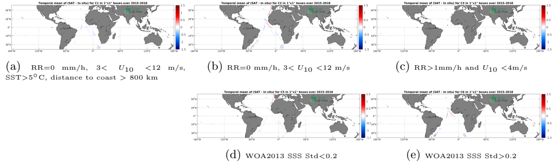
Figure 12: Temporal mean gridded over spatial boxes of size 1^\circ \times 1^\circ of \Delta SSS (SMAP SSS L3 v4 - Monthly (RSS) - TSG (Polarstern)) for 5 different subdatasets corresponding to: RR=0 mm/h, 3 < U_{10} < 12 m/s, SST>5°C, distance to coast > 800 km (a), RR=0 mm/h, 3 < U_{10} < 12 m/s (b), RR>1mm/h and U_{10} < 4 m/s (c), WOA2013 SSS Std<0.2 (d), WOA2013 SSS Std>0.2 (e).
