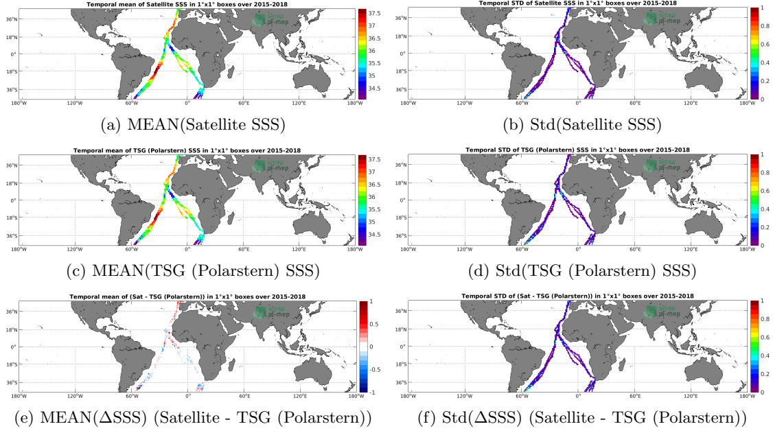
Figure 6: Temporal mean (left) and Std (right) of SSS from SMAP SSS L3 v4 - Monthly (RSS) (top), TSG (Polarstern) (middle), and of \Delta SSS (Satellite - TSG (Polarstern)). Only match-up pairs are used to generate these maps.
