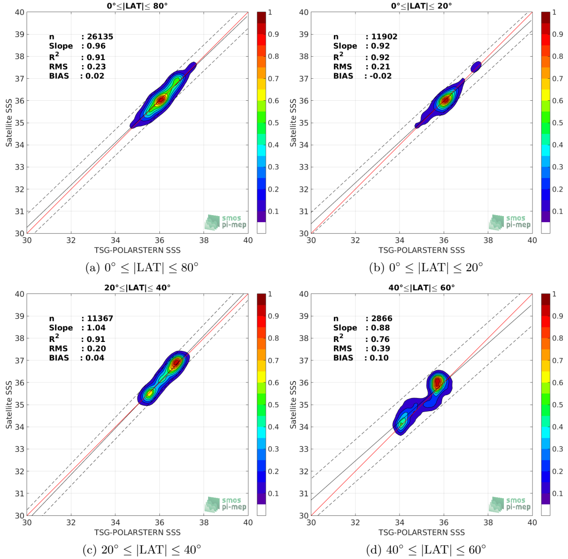
Figure 9: Contour maps of the concentration of SMAP-L3-RSS-V4-MONTHLY SSS (y-axis) versus TSG-POLARSTERN SSS (x-axis) at match-up pairs for different latitude bands. For each plot, the red line shows x=y . The black thin and dashed lines indicate a linear fit through the data cloud and the \pm 95\% confidence levels, respectively. The number match-up pairs n , the slope and R^2 coefficient of the linear fit, the root mean square (RMS) and the mean bias between satellite and in situ data are indicated for each latitude band in each plots.
